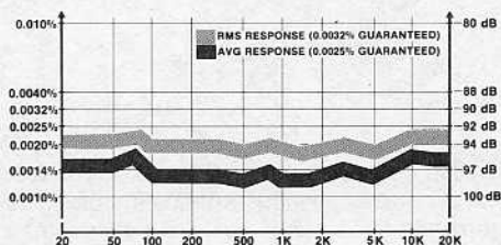
TYPICAL THD+N
