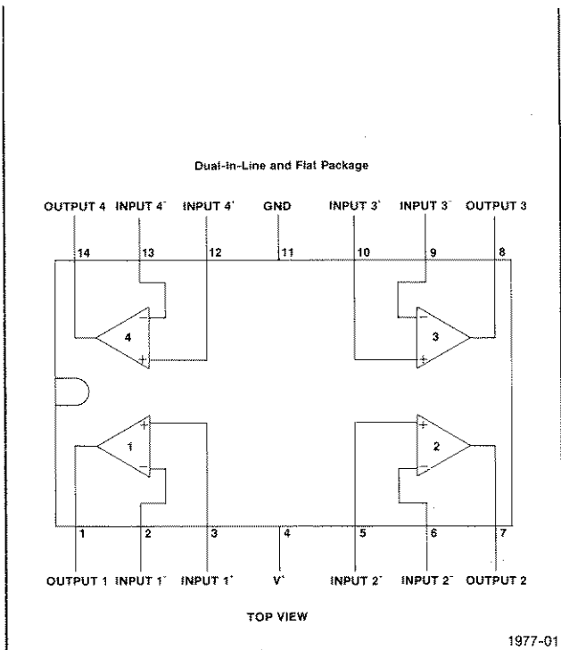
Fig. A-1. Connection diagram of the LM324.
