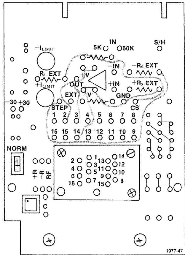
Fig. E-11. Setup for checking output sink current.
