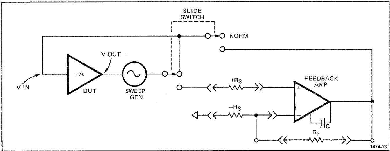
Fig. 2-10. Block diagram of the feedback amplifier.
