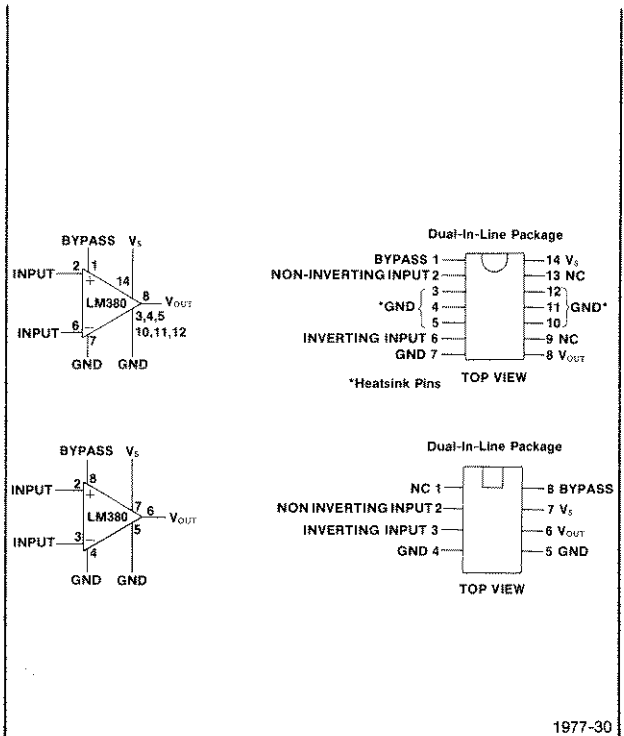
Fig. D-1. LM380 block and connection diagrams.
