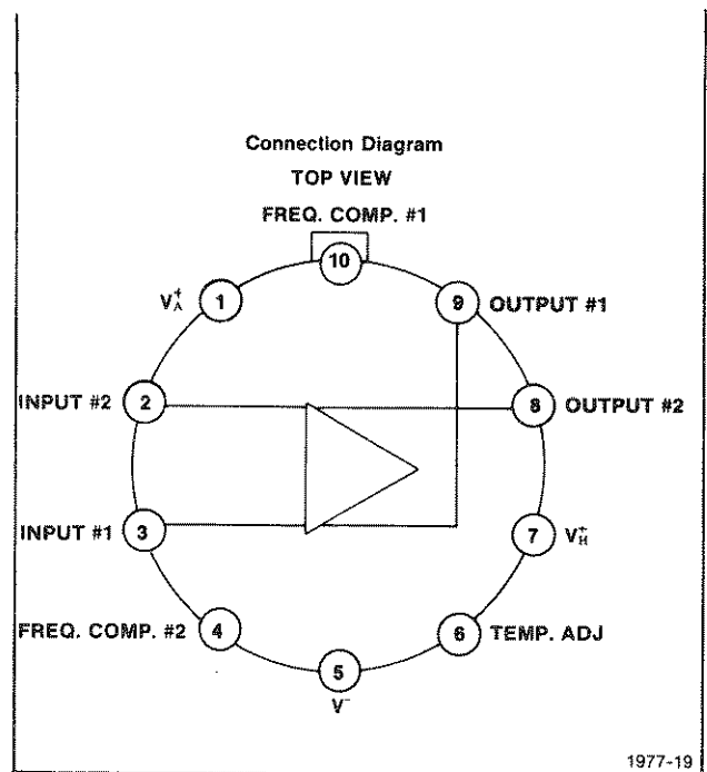
Fig. C-1. Basing and patching diagram for the 727.
