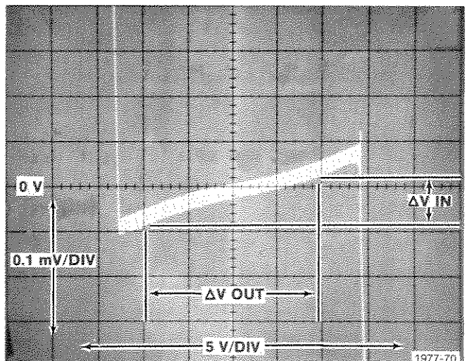
Fig. G-7. Output voltage swing.
