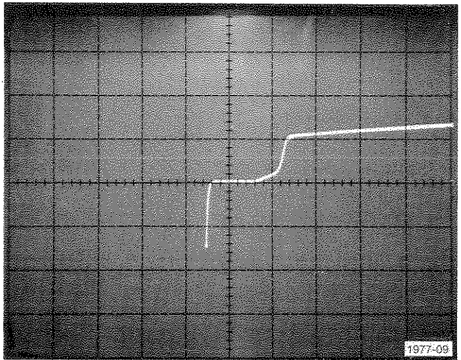
Fig. A-9. Display of maximum supply current.
