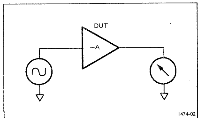
Fig. 2-2. Hypothetical open-loop test of an inverting amplifier.
