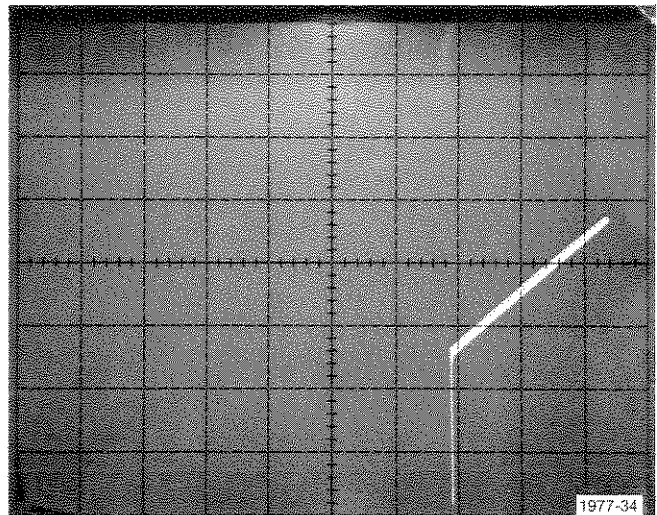
Fig. D-5. Display showing power supply rejection ratio of the LM380.
