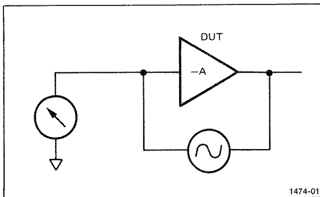
Fig. 2-1. Simplified closed-loop test of an inverting amplifier.
