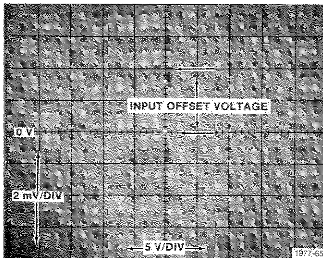
Fig. G-2. Typical display of input offset voltage.
