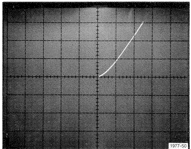
Fig. E-14. Saturation voltage.
