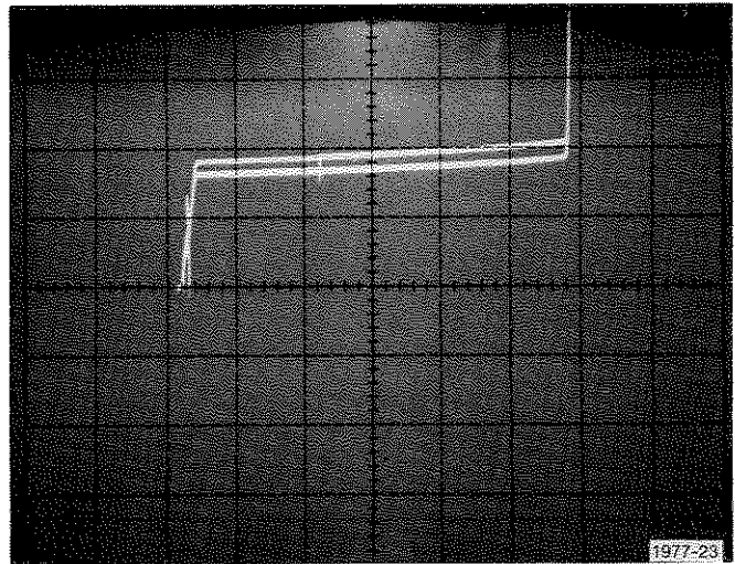
Fig. C-5. Display of input offset current.
