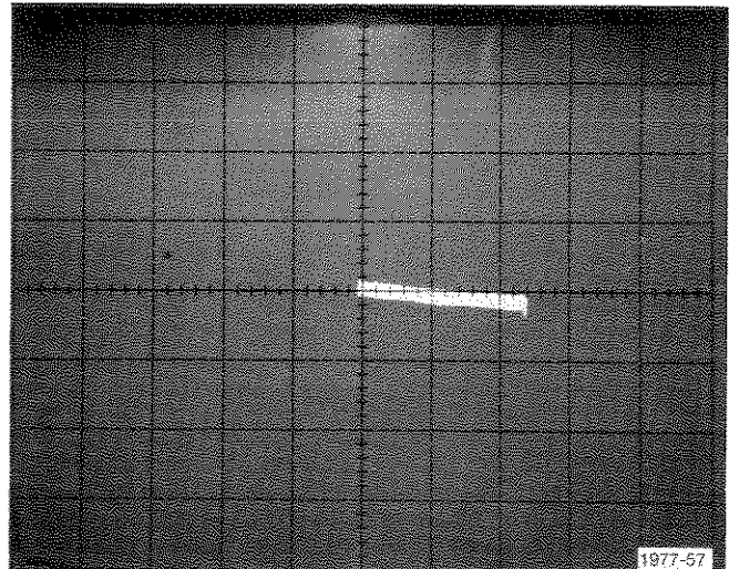
Fig. F-5. Typical display of common-mode rejection ratio.
