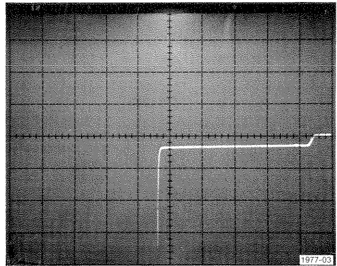
Fig. A-3. Check of LM324 + input bias current.
