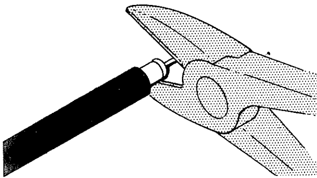
Fig. 2. The replaceable probe tip can be removed as illustrated here. Care should be taken not to squeeze or nick the grounding sleeve.
