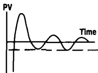
Proportional Band Too Small
