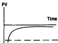
Proportional Band Too Large
