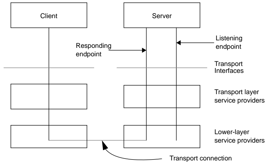
Figure 2-5 Listening and Responding Transport Endpoints
