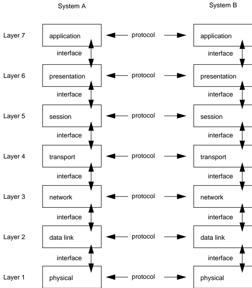
Figure 1-1 OSI Reference Model
