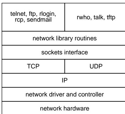
Figure 1-2 BSD Model of Network Layering
