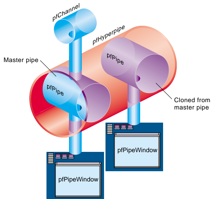
Figure 14-4 Attaching Objects to the Master pfPipe
