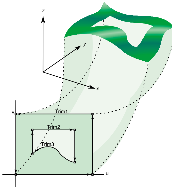
Figure 9-9 Trim Loops and Trimmed Surface: Both Trim Loops Made of Four Trim Curves
