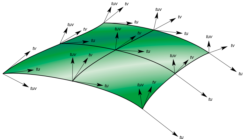
Figure 9-19 Hermite Spline Surface With Derivatives Specified at Knot Points
