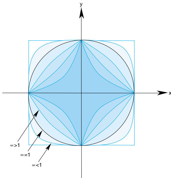
Figure 9-5 Superquadric Curve's Dependence on the Parameter \alpha .
