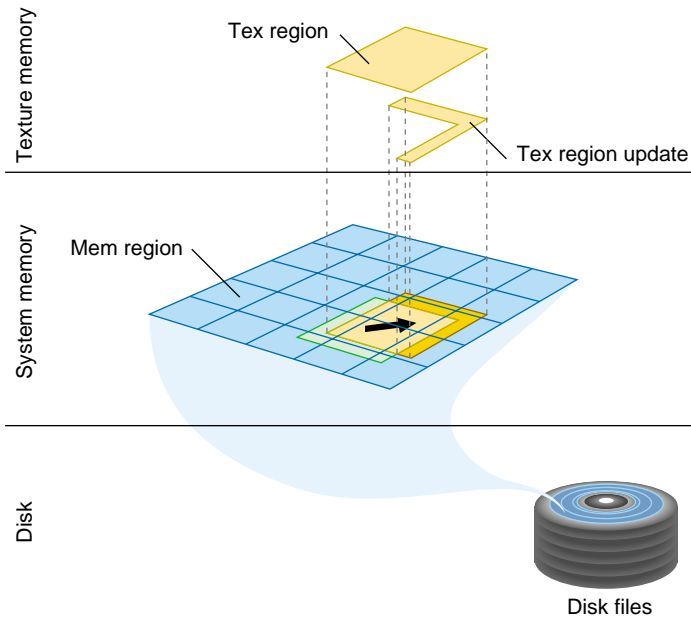
Figure 15-4 Tex Region Update
