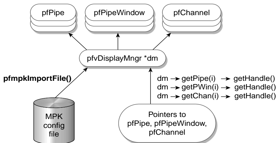
Figure 2-7 The libpfmpk Import Operation
