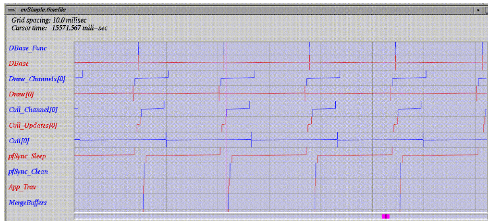
Figure 24-1 The evanalyzer Main Display
