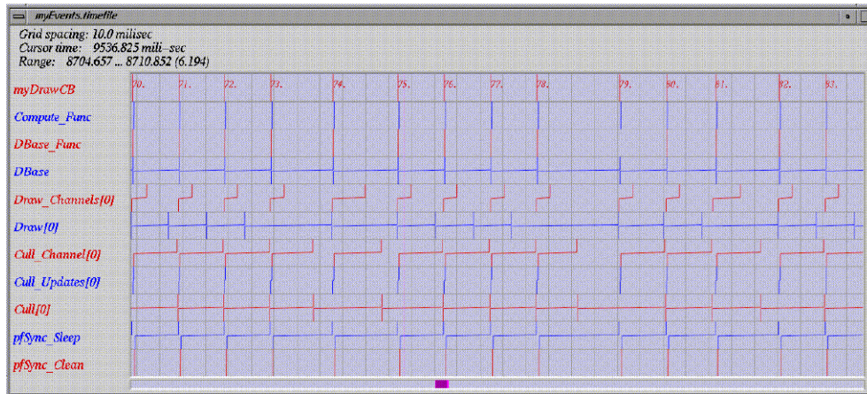
Figure 24-2 User Event myDrawCB
