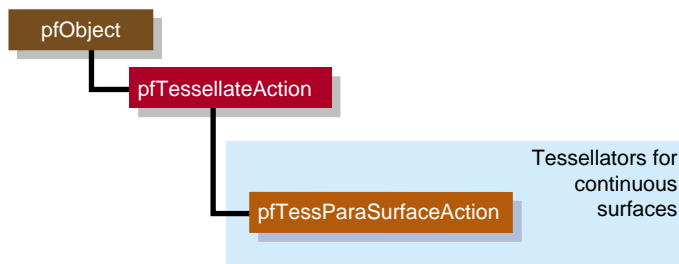
Figure 11-1 Class Hierarchy for Tessellators
