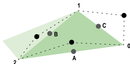
Figure 20-13 Vertex and Reference Point Arrays, Counter-Clockwise Ordering
