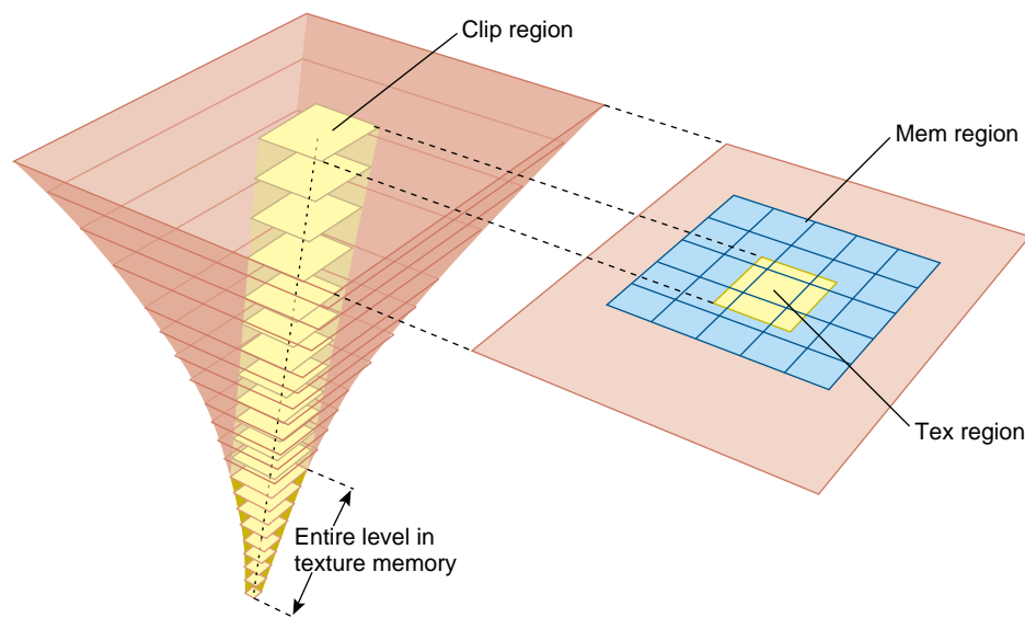
Figure 15-2 Image Cache Components
