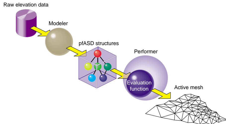
Figure 20-3 ASD Information Flow
