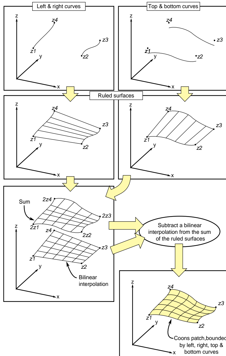
Figure 9-17 Coons Patch Construction
