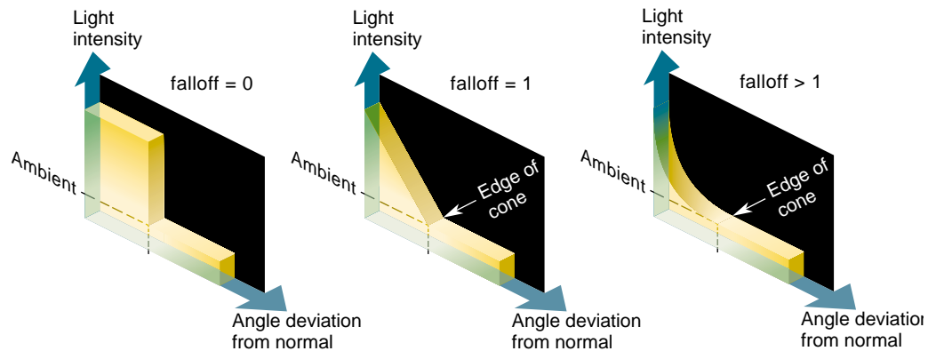
Figure 21-3 Attenuation of Light
