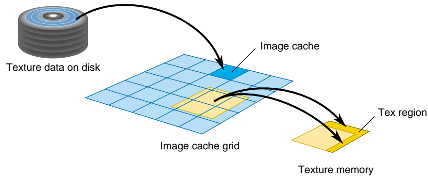
Figure 15-5 Cliptexture Cache Hierarchy
