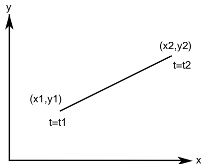
Figure 9-3 Line in the Plane Parameterization
