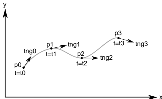
Figure 9-6 Hermite Spline Curve Parameterization
