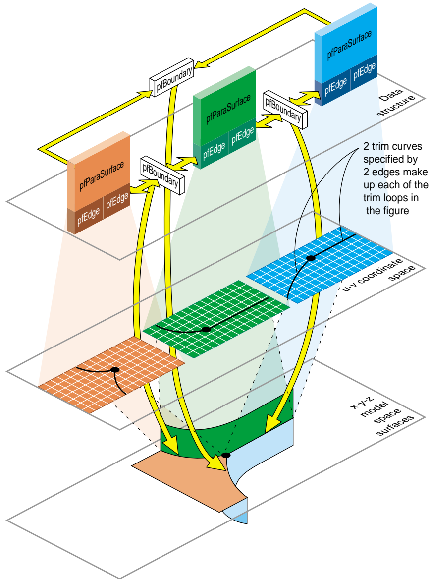
Figure 10-1 Topological Relations Maintained by Topology Classes
