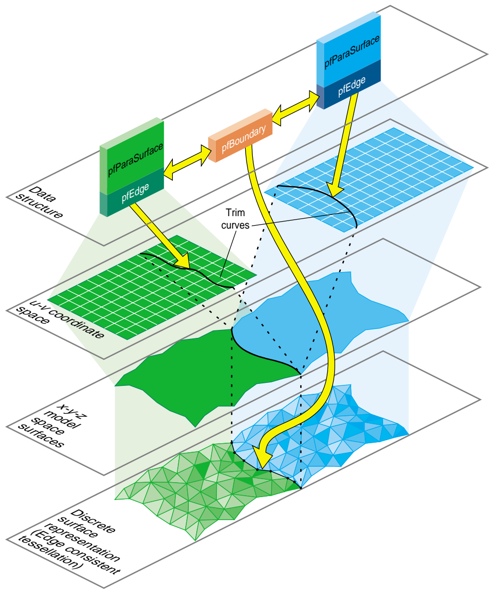
Figure 10-2 Consistently Tessellated Adjacent Surfaces and Related Objects
