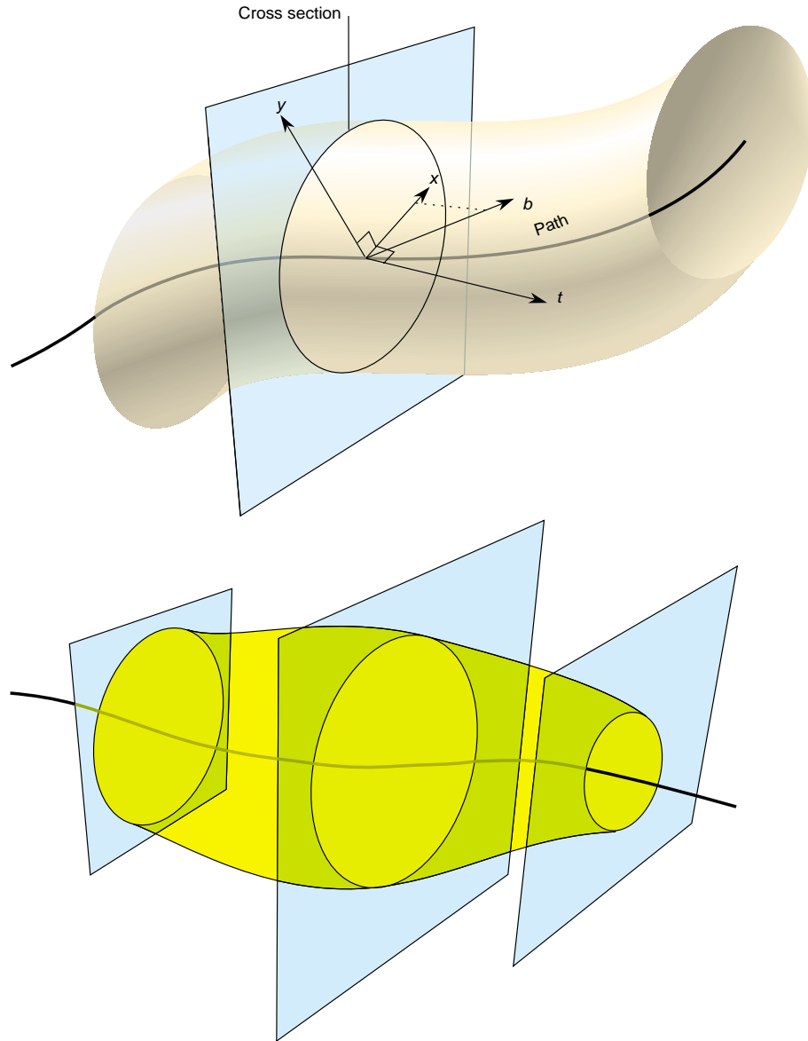
Figure 9-15 Swept Surface: Moving Reference Frame and Effect of Profile Function
