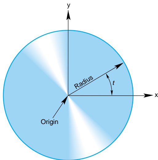
Figure 9-4 Circle in the Plane Parameterization
