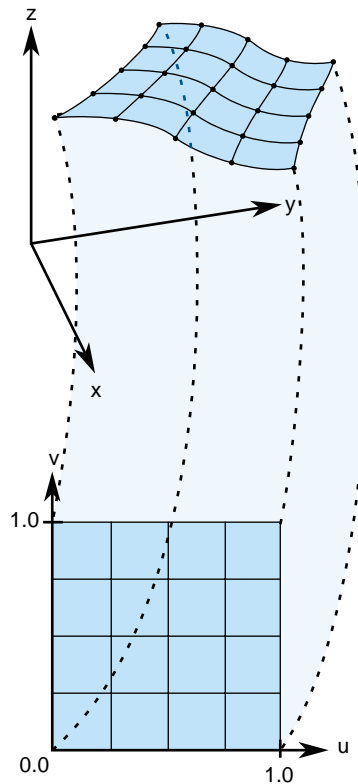
Figure 9-8 Parametric Surface: Unit-Square Coordinate System
