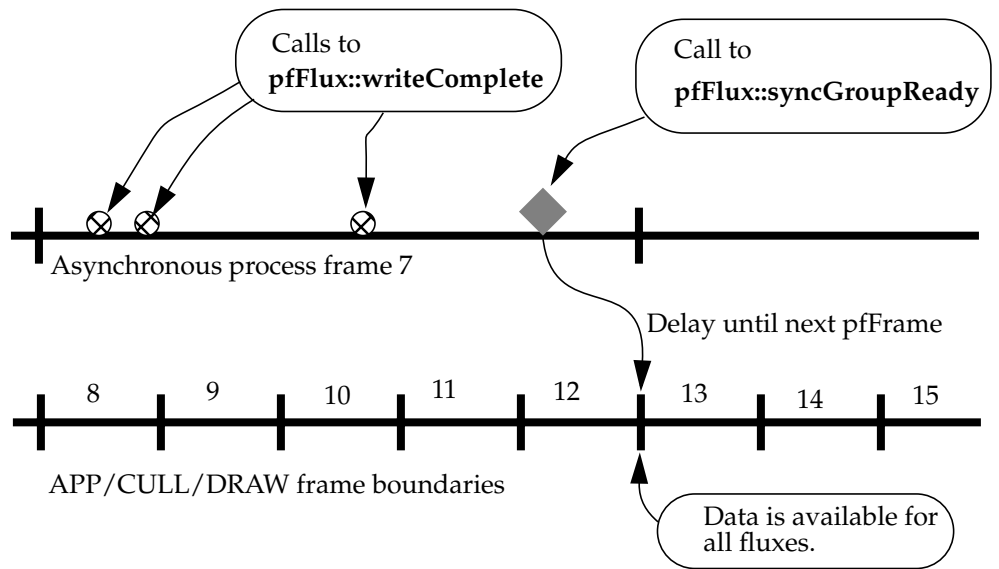
Figure 19-3 Timing Diagram Showing the Use of Sync Groups
