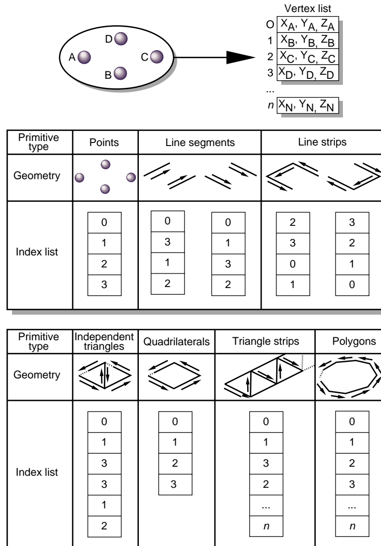
Figure 8-1 Primitives and Connectivity
