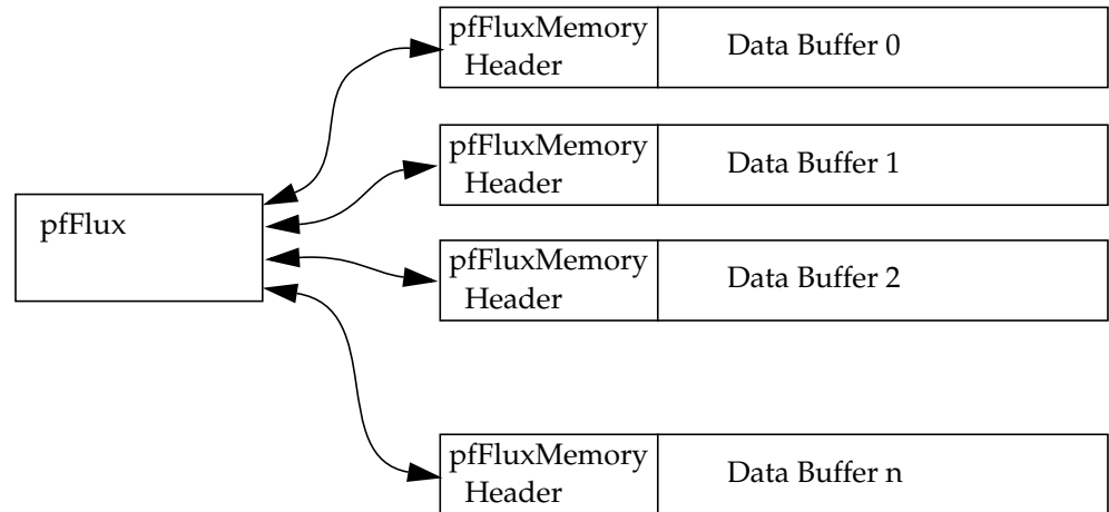
Figure 19-2 pfFlux Buffer Structure
