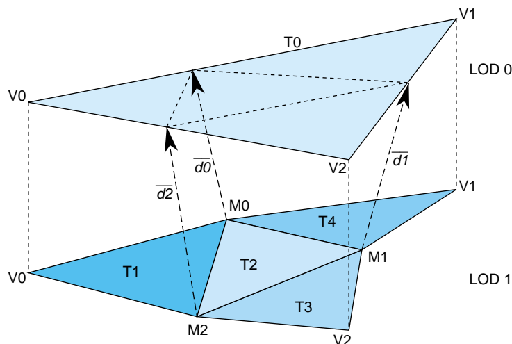
Figure 20-4 A Very Simple pfASD
