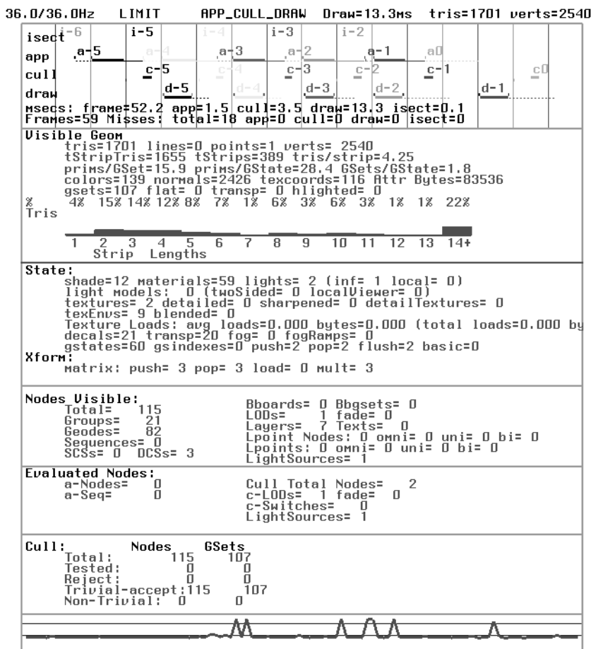
Figure 23-3 Other Statistics Classes
