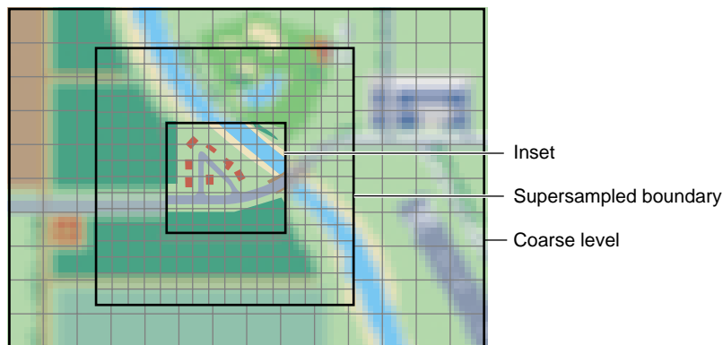
Figure 15-13 Supersampled Inset Boundary
