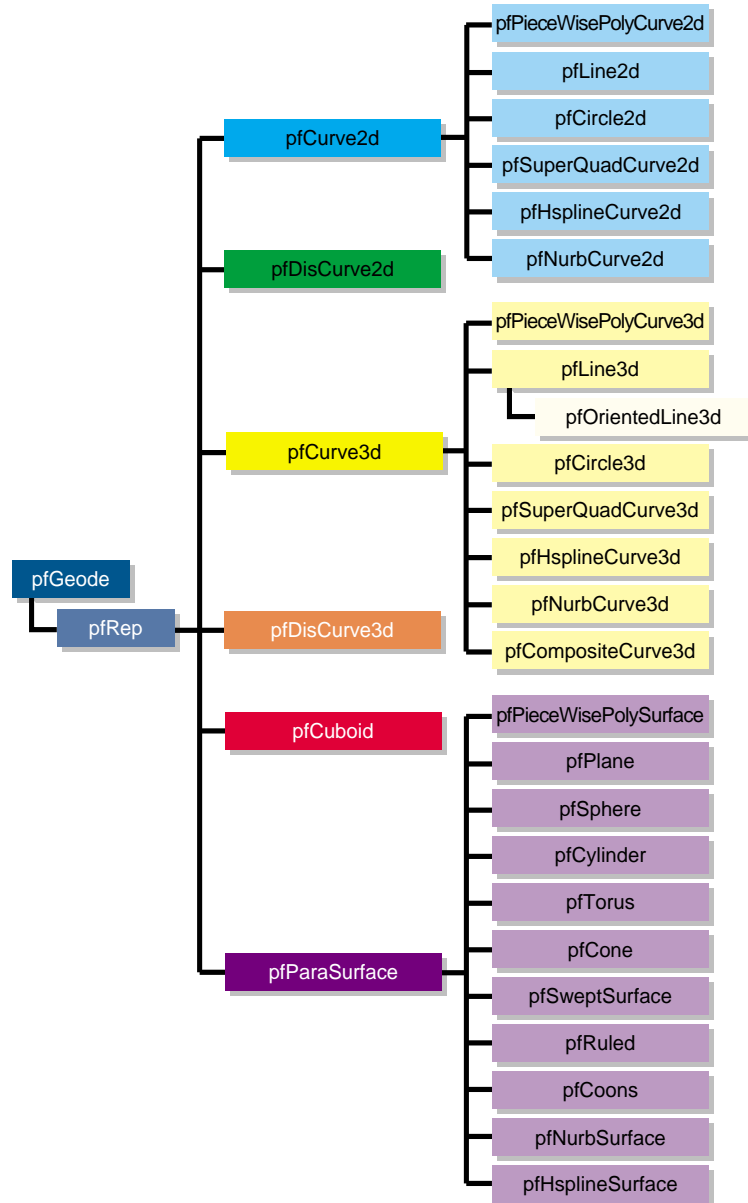
Figure 9-1 Class Hierarchy for Higher-Order Primitives
