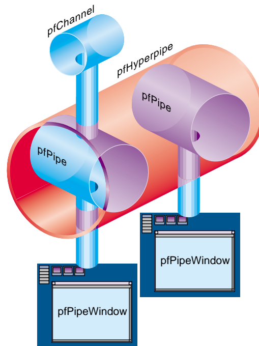
Figure 14-1 pfPipes Creating pfHyperpipes
