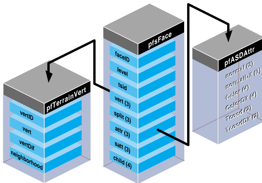
Figure 20-9 ASD Data Structures
