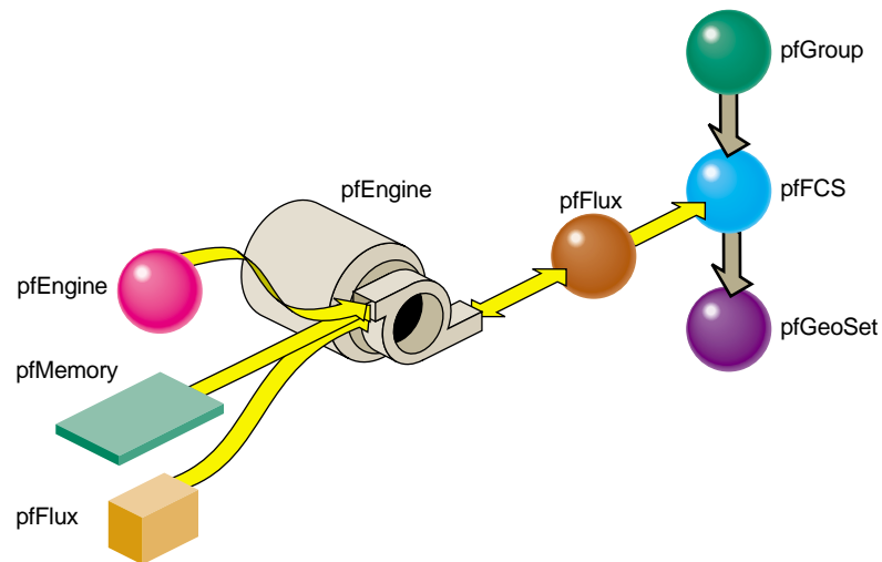
Figure 19-4 pfEngine Driving a pfFlux That Animates a pfFCS Node
