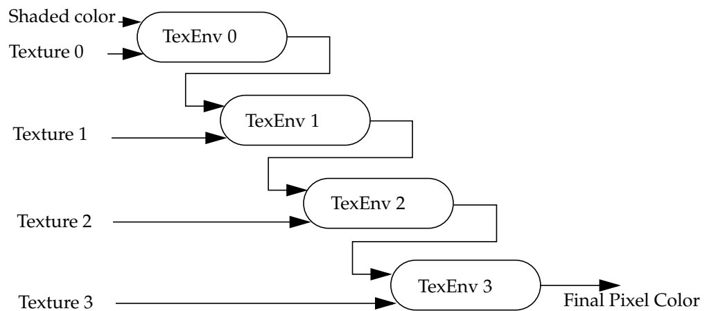
Figure 12-2 Generating the Color of a Multitextured Pixel
