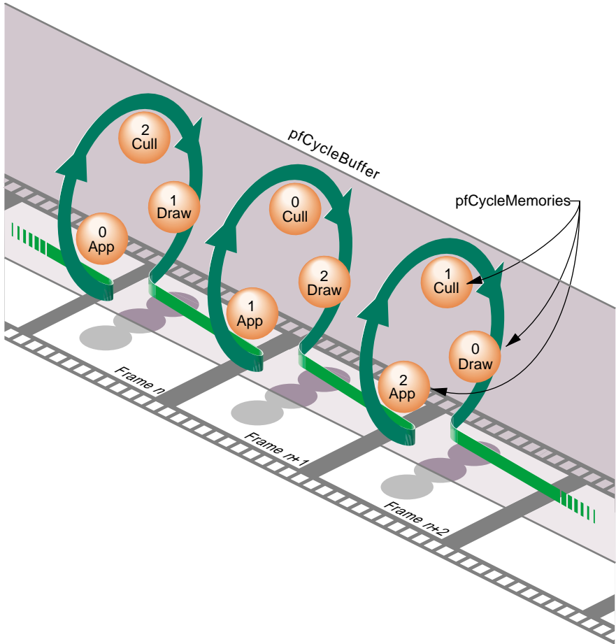
Figure 18-2 pfCycleBuffer and pfCycleMemory Overview
