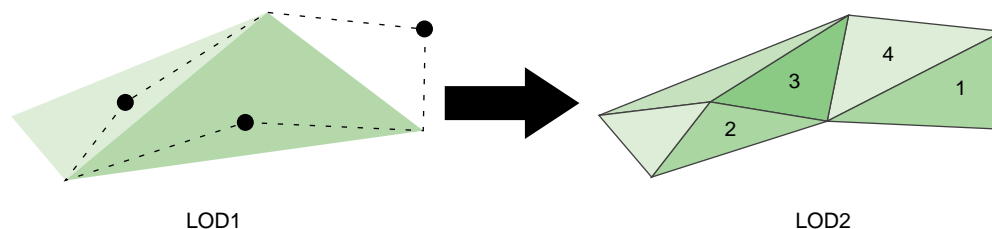
Figure 20-7 LOD1 Replaced by LOD2
