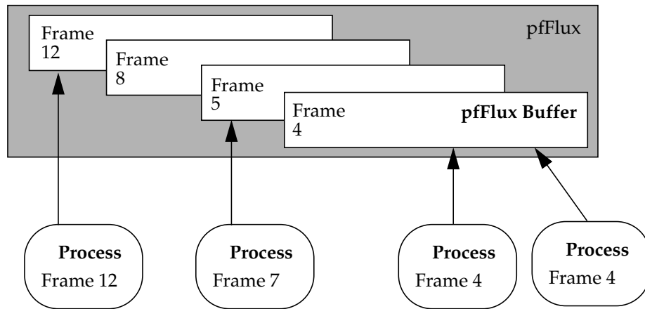
Figure 19-1 How pfFlux and Processes Use Frame Numbers
