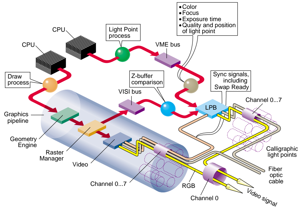
Figure 21-5 Calligraphic Hardware Configuration
