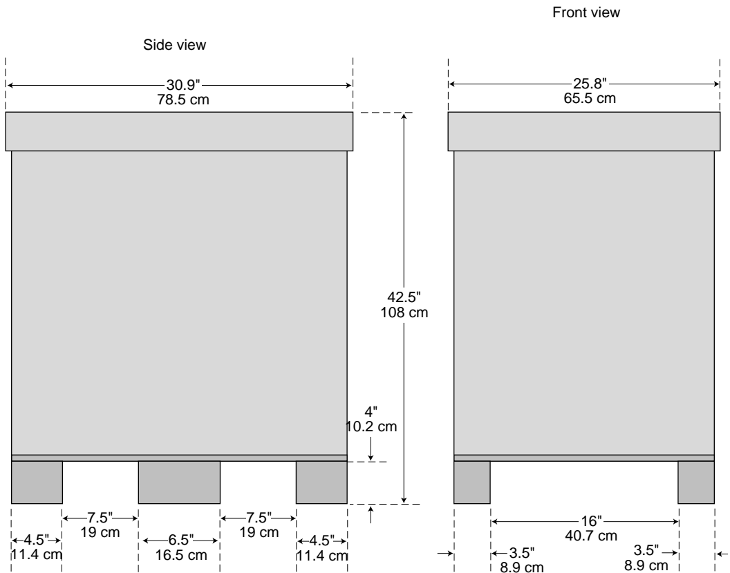
Figure 6-1 SGI 2000-Series Deskside and Onyx2 Deskside Shipping Crate
