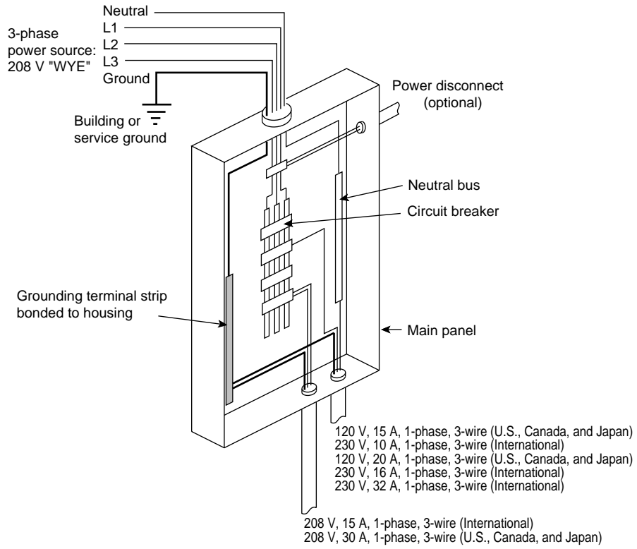
Figure B-1 Main Circuit Wiring
