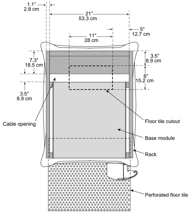
Figure 8-8 SGI 2000-Series, Origin Peripherals, and Onyx2 Rack-Chassis Cable Opening, Raised-Floor Cutout, and Perforated Tile
