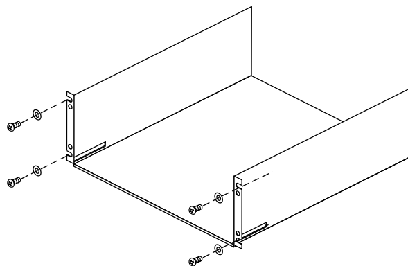
Figure 5-3 Origin200 and Origin Vault Rack Shelf and Mounting Hardware
