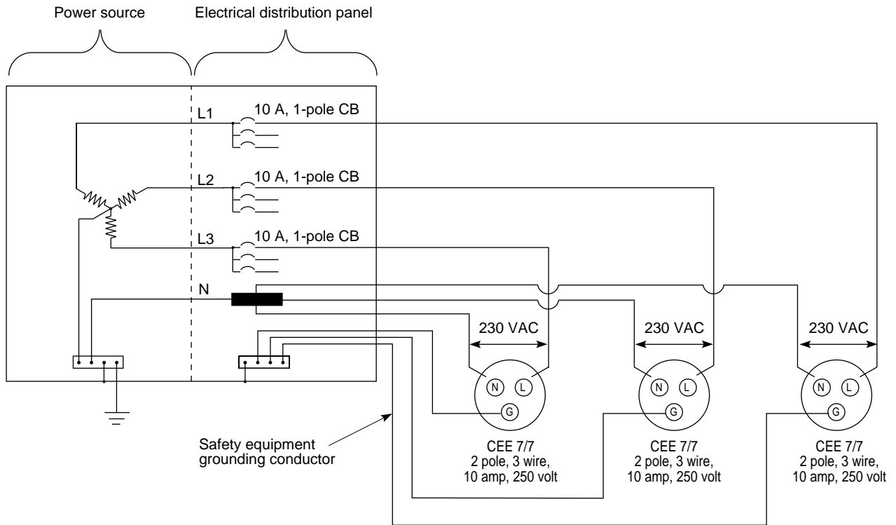
Figure B-4 Chassis Branch Circuit Diagram for 230 VAC, 10 amp, 3-wire, 1-phase (International)
