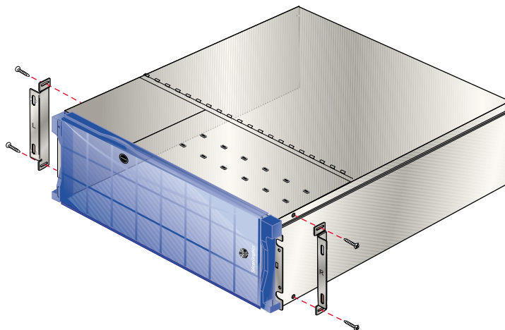
Figure 5-2 Origin200 and Origin Vault Rack-Mount Configuration and Mounting Hardware
