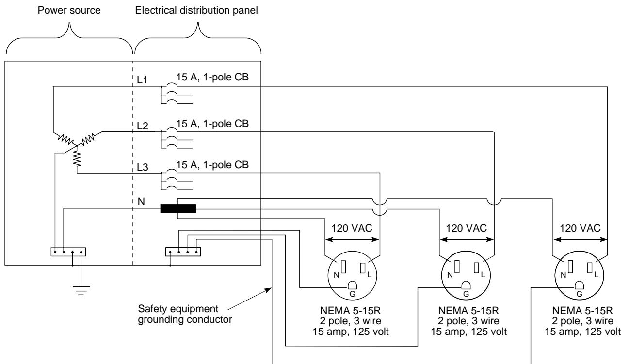
Figure B-3 Chassis Branch Circuit Diagram for 120 VAC, 15 amp, 3-wire, 1-phase (U.S., Canada, and Japan)
