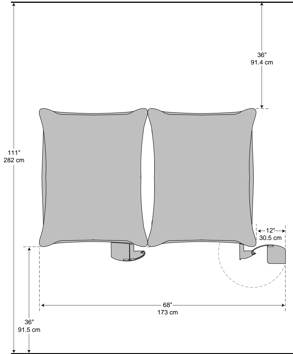
Figure 8-9 Two-Chassis SGI 2000-Series, Origin Peripherals, or Onyx2 Rack Recommended Clearances
