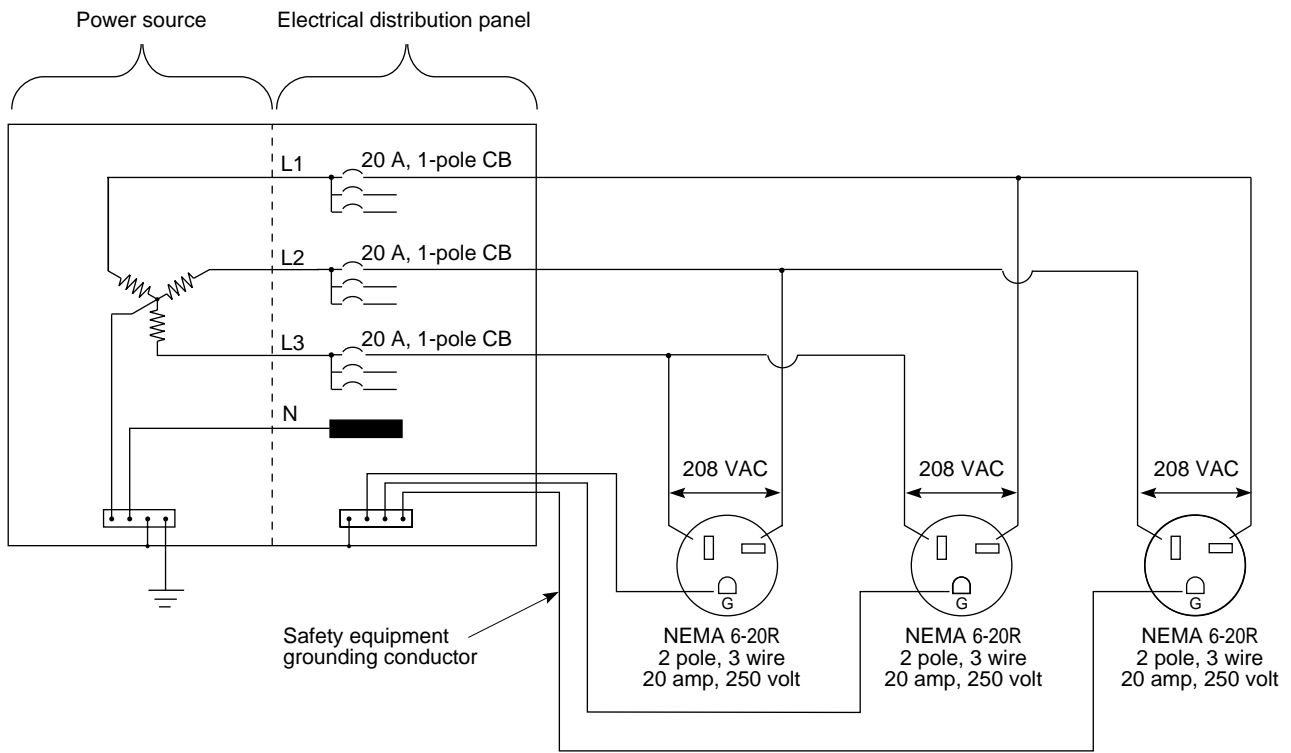
Figure B-6 Chassis Branch Circuit Diagram for 208 VAC, 20 amp, 3-wire, 1-phase (U.S., Canada, and Japan)
