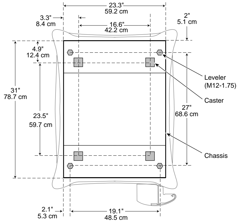
Figure 8-4 SGI 2000-Series Origin2000, Origin Peripherals, and Onyx2 Rack Chassis Caster and Leveler Locations
