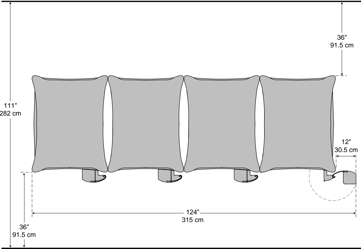
Figure 8-10 Four-Chassis SGI 2000-Series, Origin Peripherals, or Onyx2 Rack Recommended Clearances
