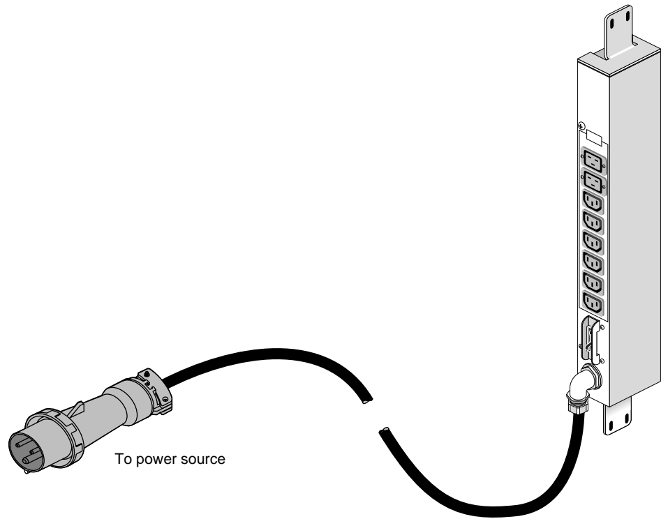
Figure B-20 SGI 2000-Series and Onyx2 Rack Power Cable, 250 VAC, 32 A (International)
