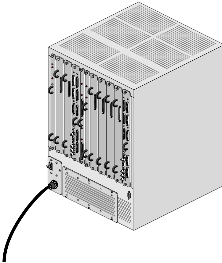
Figure 7-1 Onyx2 Graphics Insert Module, Rear View
