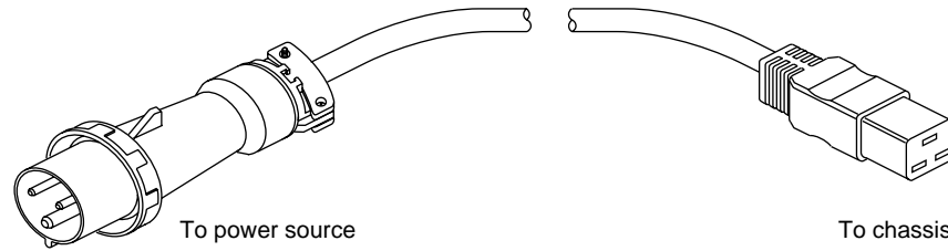
Figure B-15 SGI 2000-Series Deskside and Onyx2 Deskside Power Cable, 250 VAC, 16 A (International)
