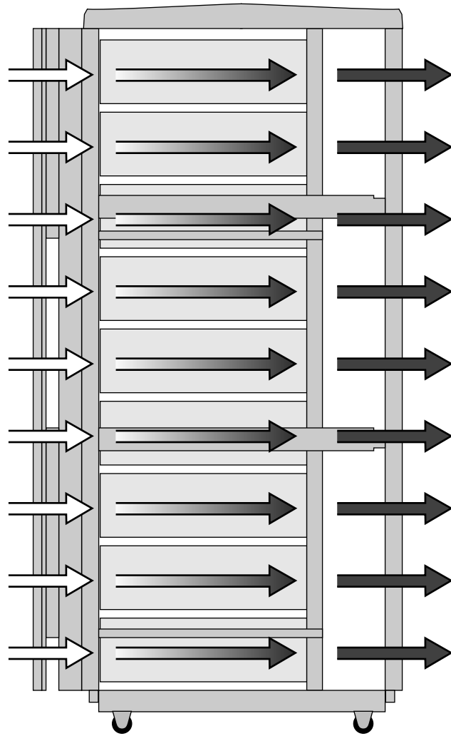
Figure 8-7 Origin Peripherals Rack-Chassis Airflow (Shown With the Maximum of Nine Origin200 or Origin Vault Units)
