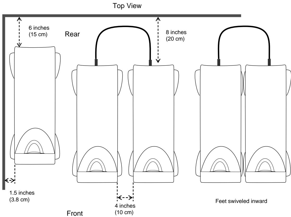
Figure 5-4 Origin200 and Origin Vault Chassis Clearances
