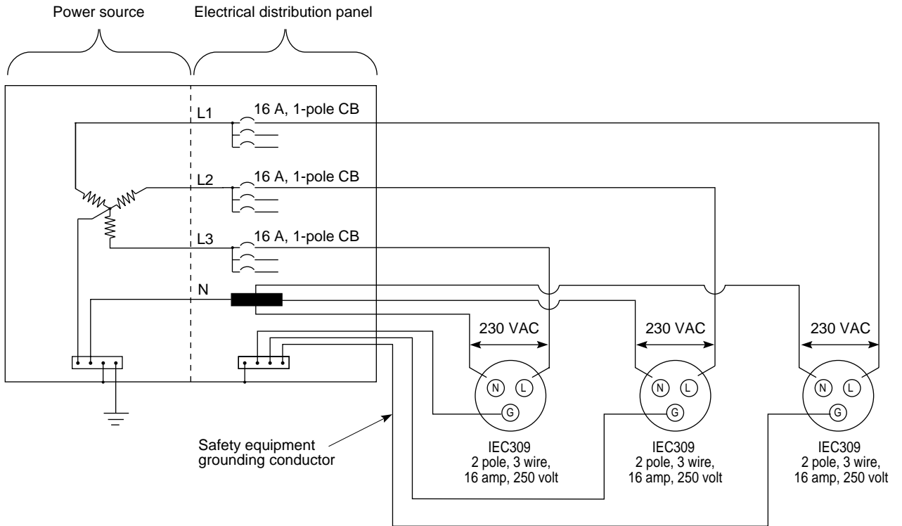
Figure B-7 Chassis Branch Circuit Diagram for 230 VAC, 16 amp, 3-wire, 1-phase (International)
