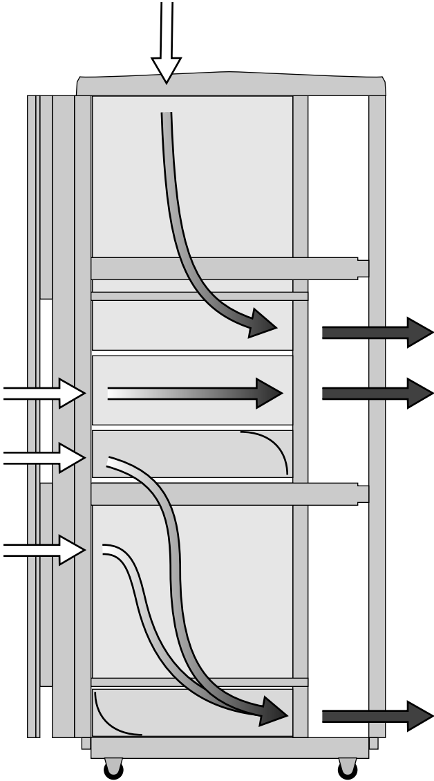
Figure 8-6 Onyx2 Rack-Chassis Airflow (Shown With One Base Module, One Onyx2 Graphics Insert Module, and One Origin Vault)
