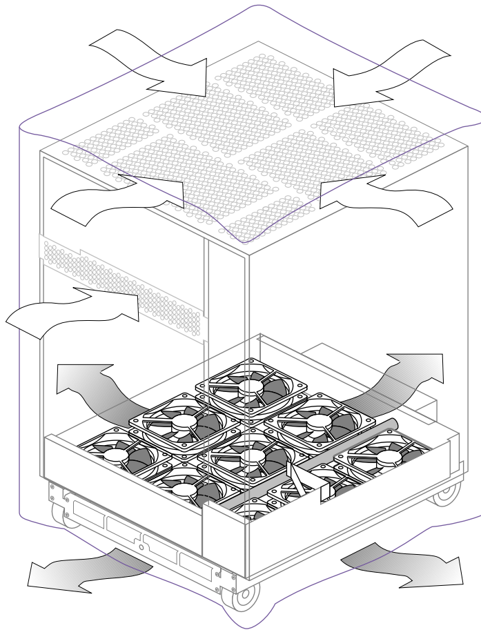
Figure 6-3 SGI 2000-Series Deskside and Onyx2 Deskside Airflow
