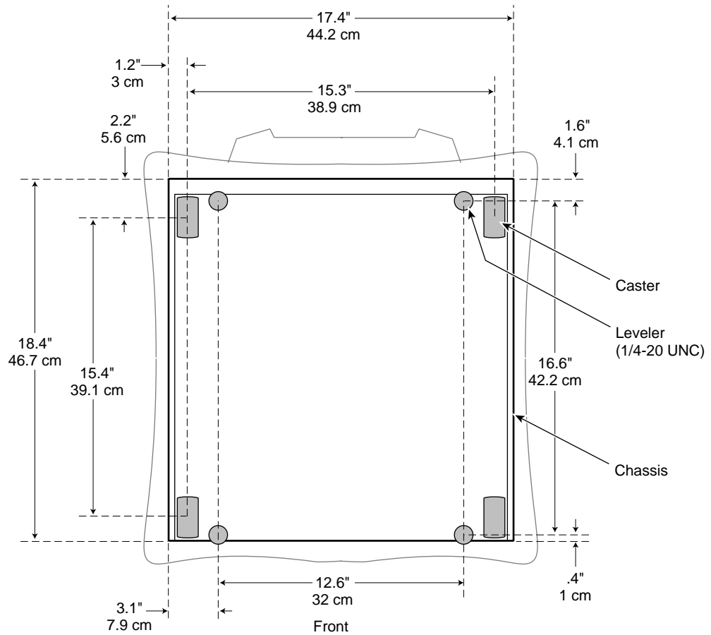
Figure 6-4 SGI 2000-Series Deskside and Onyx2 Deskside Caster Positions
