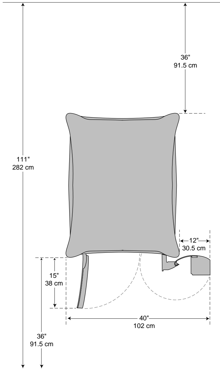
Figure 8-3 SGI 2000-Series, Origin Peripherals, and Onyx2 Rack Chassis Recommended Clearances
