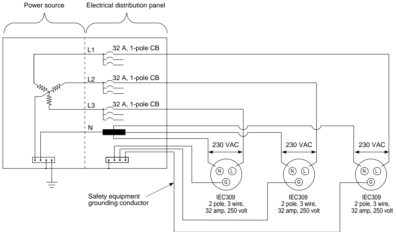
Figure B-9 Chassis Branch Circuit Diagram for 230 VAC, 32 amp, 3-wire, 1-phase (International)
