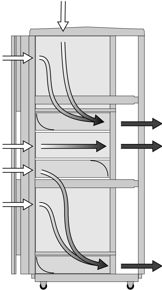
Figure 8-5 SGI 2000-Series Rack-Chassis Airflow (Shown With Two Base Modules and One Origin Vault)
