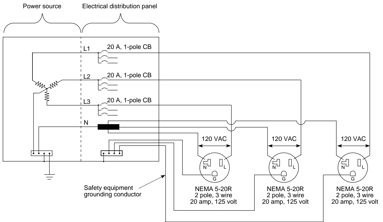
Figure B-5 Chassis Branch Circuit Diagram for 120 VAC, 20 amp, 3-wire, 1-phase (U.S. and Canada)
