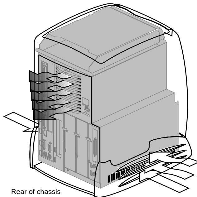
Figure 3-2 O2 Airflow
