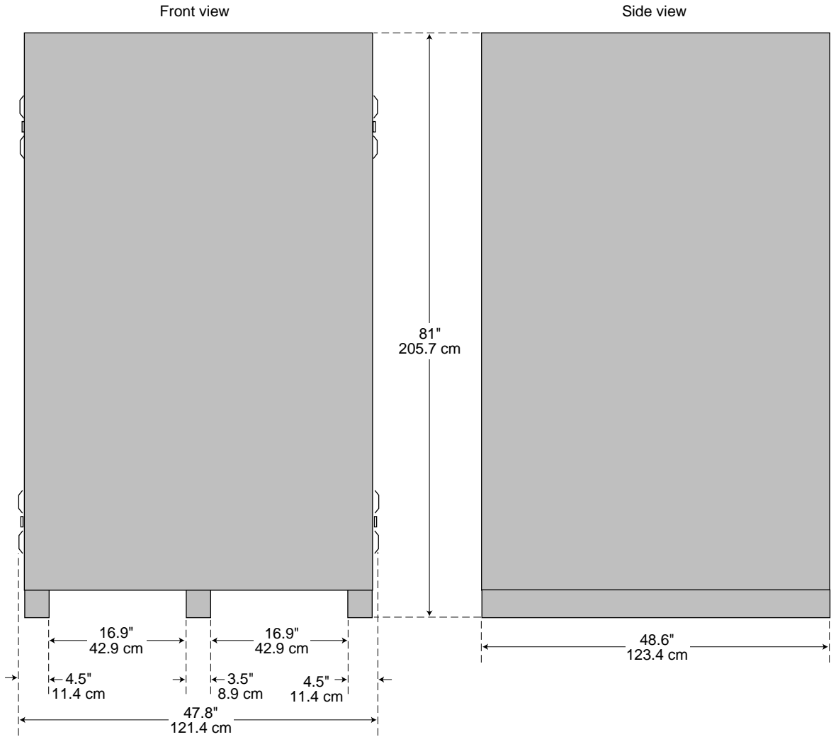
Figure 8-1 SGI 2000-Series, Origin Peripherals, and Onyx2 Rack Chassis Shipping Crate
