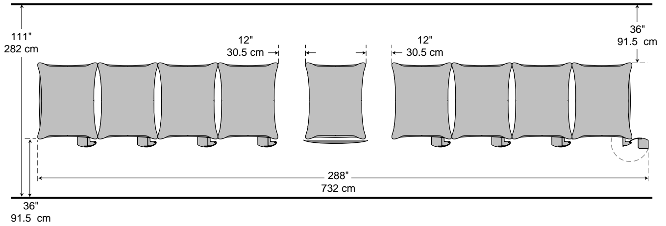
Figure 8-11 Nine-Chassis SGI 2000-Series or Onyx2 Rack Recommended Clearances (Center Chassis is a Meta-Router)
