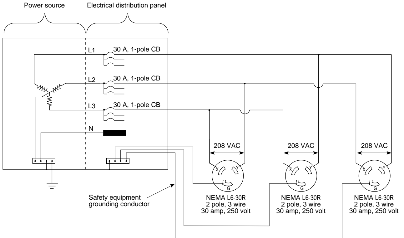
Figure B-8 Chassis Branch Circuit Diagram for 208 VAC, 30 amp, 3-wire, 1-phase (U.S., Canada, and Japan)
