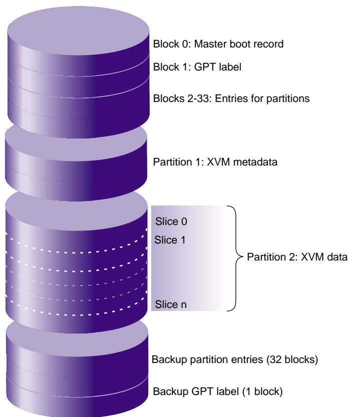
Figure 1-5 GPT Disk Layout for XVM
