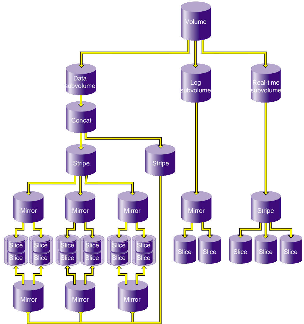
Figure 1-9 XVM Logical Volume after Insertion of Concat
