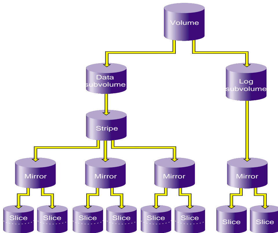
Figure 1-8 XVM Logical Volume with Mirrored Stripe and Three Subvolumes
