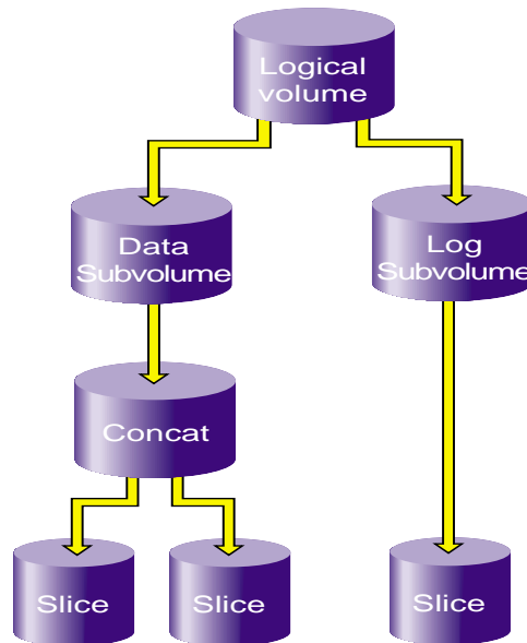
Figure 6-4 Logical Volume with Data and Log Subvolumes
