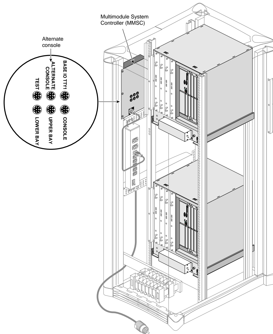
Figure F-10 MMSC Serial Port
