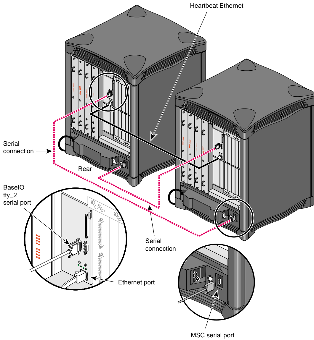
Figure F-9 Serial Connection Between Two SGI 2200 Deskside Servers
