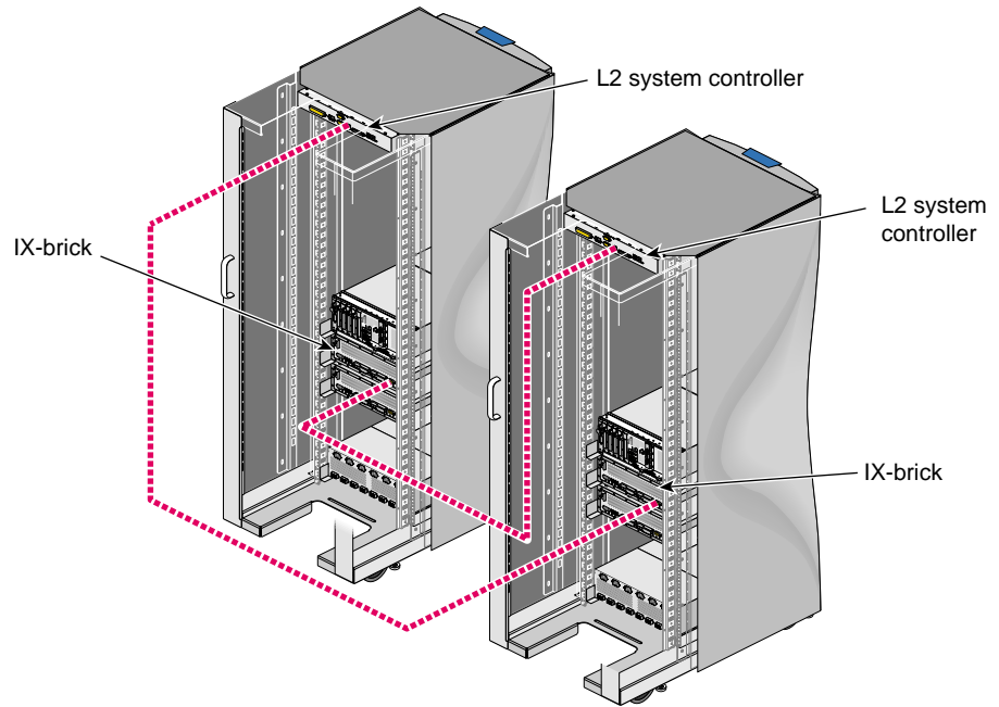
Figure F-6 Serial Connection Between Two SGI Origin 3400 or SGI Origin 3800 Servers
