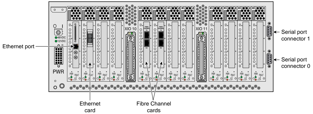
Figure F-3 IX-brick Rear Panel
