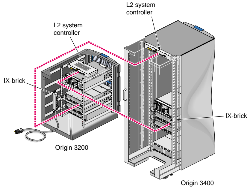
Figure F-5 Serial Connection Between SGI Origin 3200 and Origin 3400/3800 Servers
