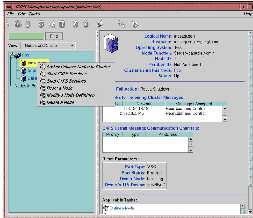
Figure 9-2 Pop-up Menu that Appears After Clicking the Right Mouse Button
