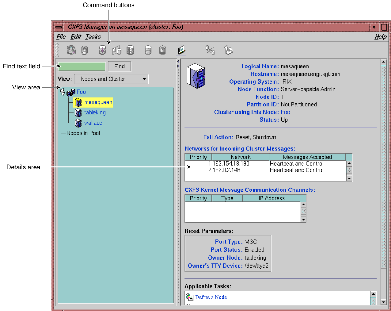
Figure 9-1 CXFS Manager GUI Showing Details for a Node
