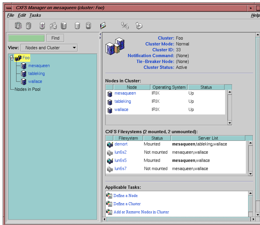
Figure 8-1 CXFS Manager
