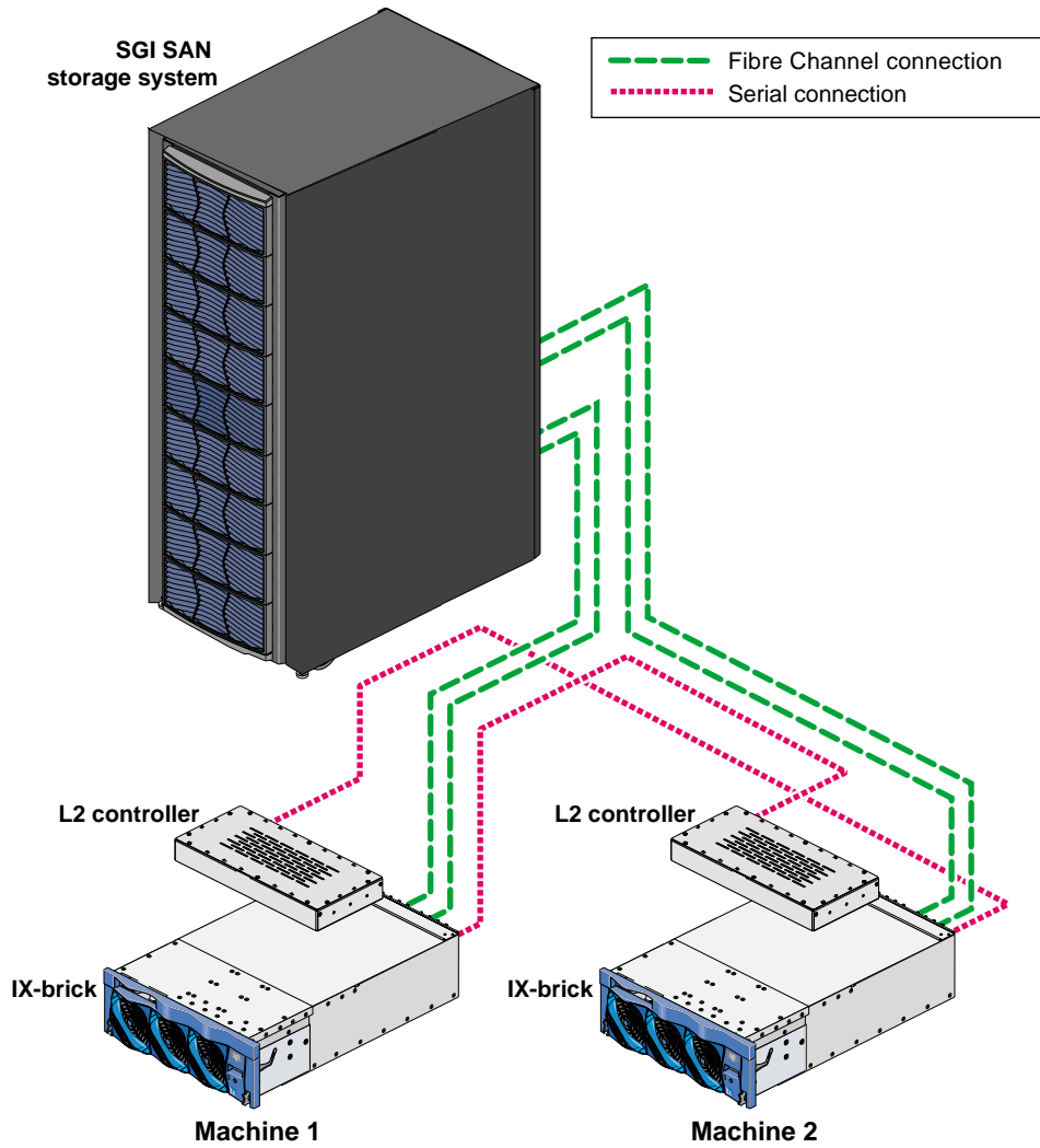
Figure F-4 Altix 3000 and Origin 3000 Serial Connections
