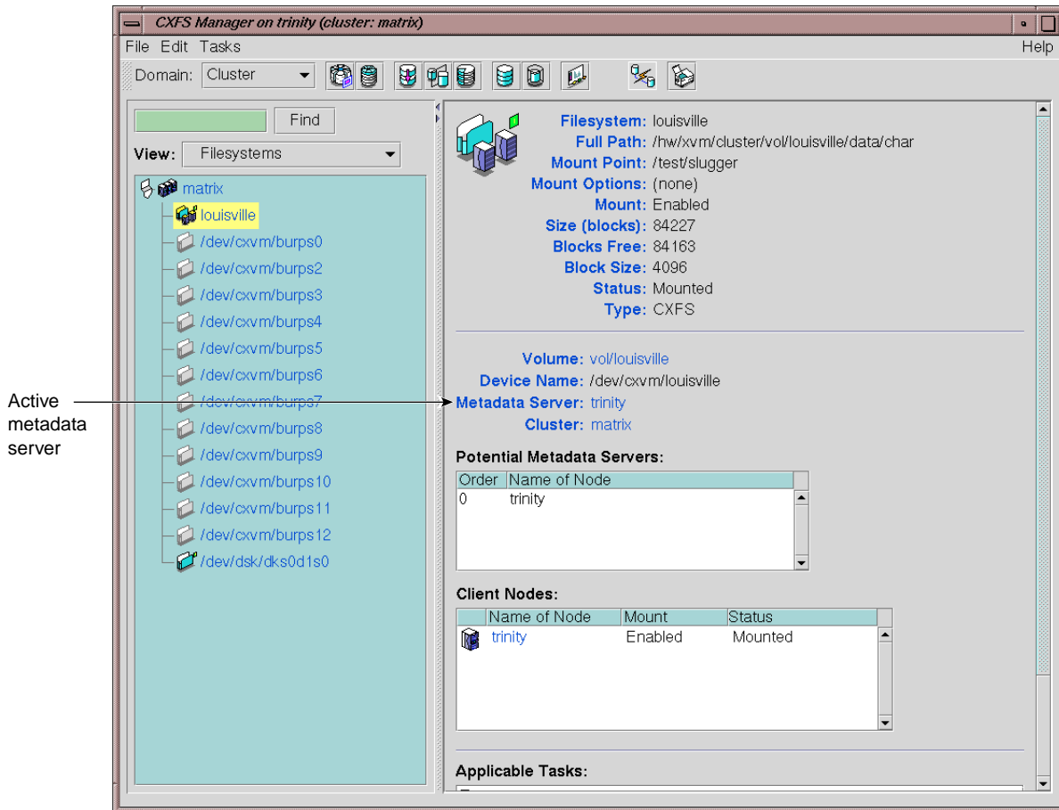
Figure 11-1 Window Showing the Metadata Server
