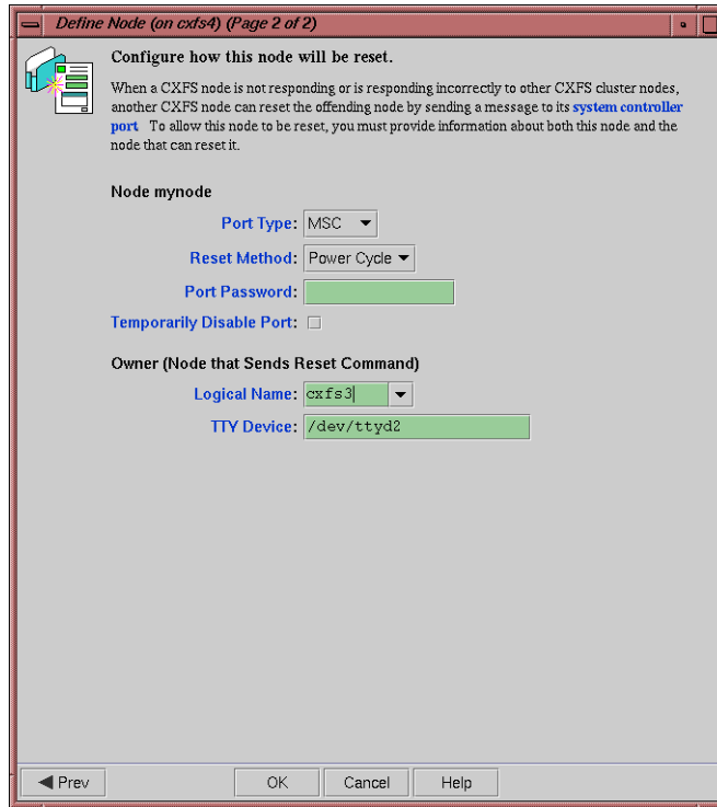
Figure 9-4 Example System Reset Settings
