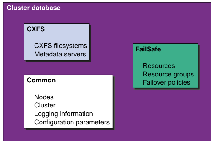
Figure 1-9 Contents of a Coexecution Cluster Database
