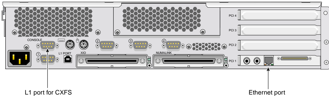
Figure F-7 Origin 350 Rear Panel
