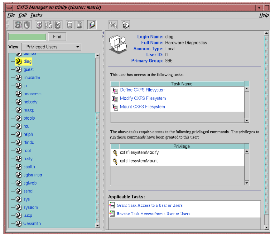
Figure 9-6 Task Privileges for a Specific User
