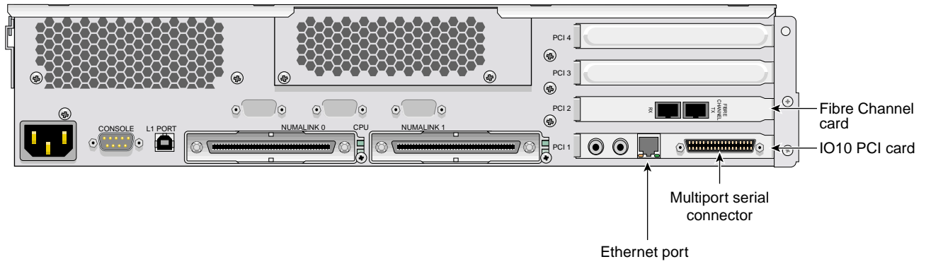
Figure F-1 Altix 350 Rear Panel
