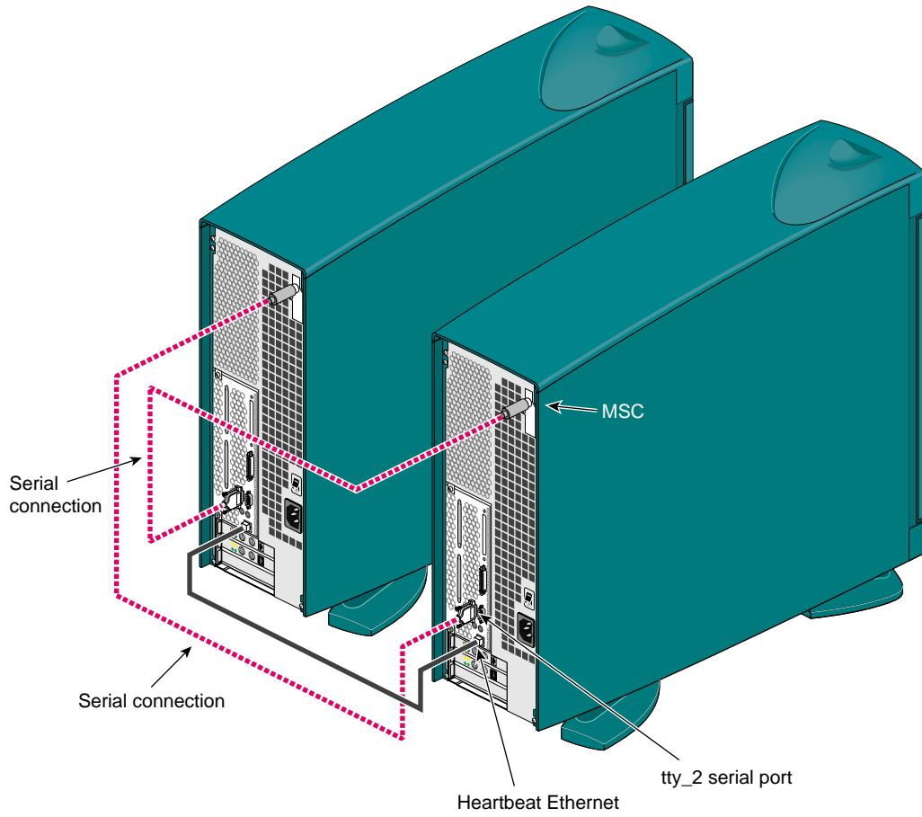
Figure F-8 Serial Connection Between Two Origin 200 Deskside Servers
