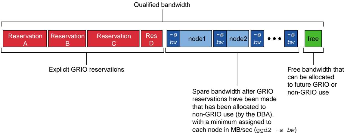
Figure 2-1 Qualified Bandwidth
