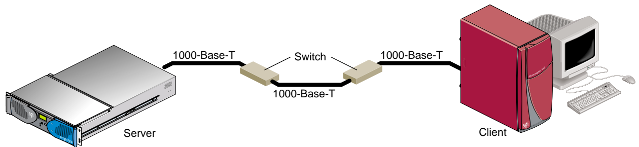
Figure 1-5 Example of 1000-Base-T Configuration
