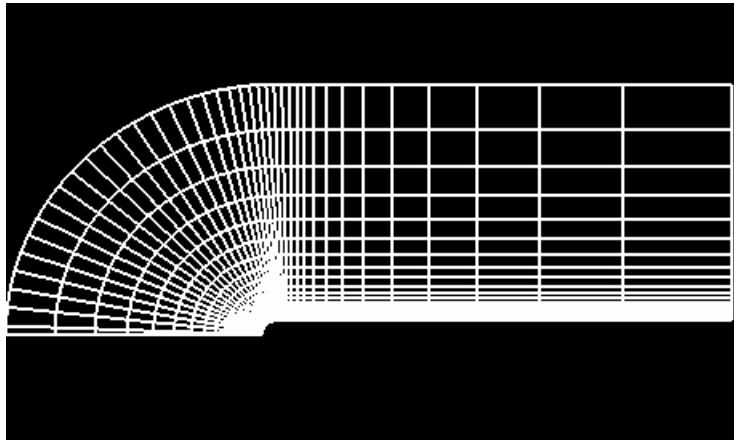
Figure 7-1 Blunt Fin Dataset (Wireframe Model)
