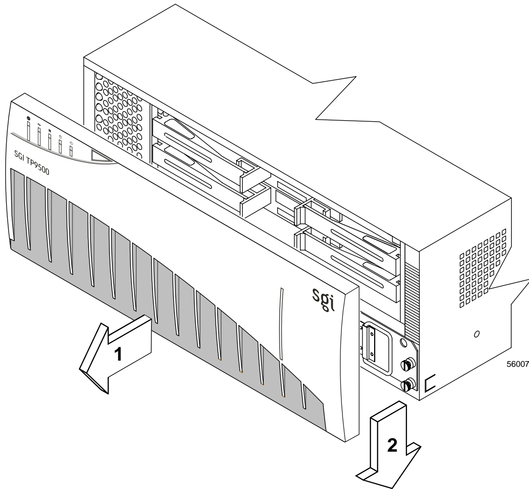
Figure 2-4 Removing the Front Panel of the SGI InfiniteStorage TP9500 Controller Enclosure
