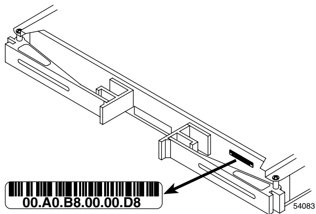
Figure 2-5 Identifying the Controller Ethernet Address on the SGI InfiniteStorage TP9500 RAID Controller
