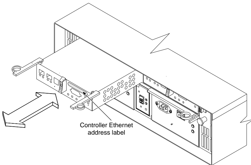
Figure 2-6 Identifying the Controller Ethernet address on the SGI InfiniteStorage TP9300 RAID Controller
