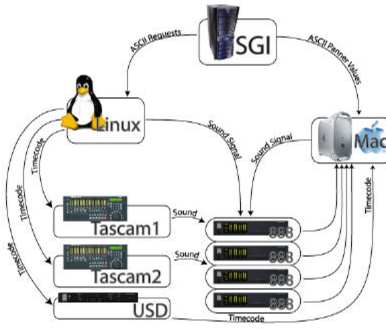
Figure 1: Control Flow
