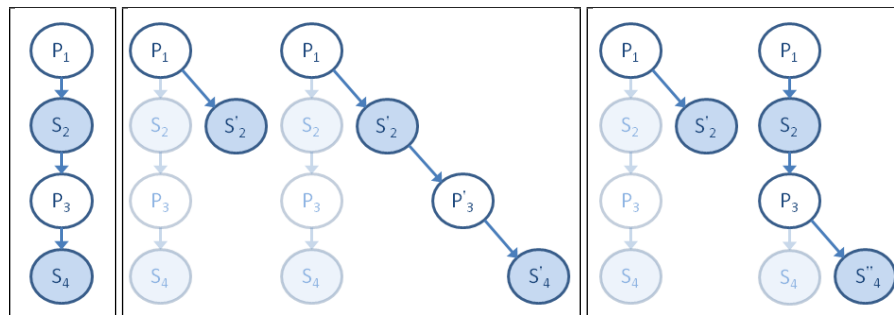
(a) Original human-human dialogue (b) Dynamic Context Setting (c) Static Context Setting
