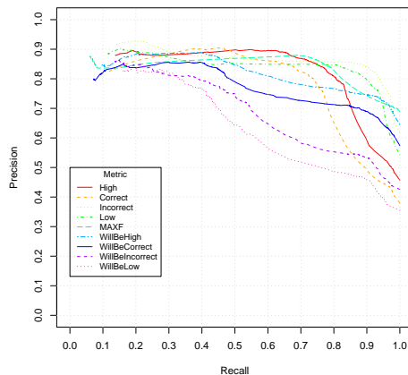
Figure 4: Precision vs. Recall for Incremental Classification Metrics
