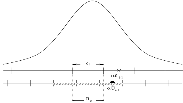
Figure 2: Overlapping shifted quantizers. Using information from the coarse reproduction the number of potential bins for Q_f is reduced. Only the bins of Q_f which overlap the region R_c are valid. The valid bins of Q_f are highlighted.
