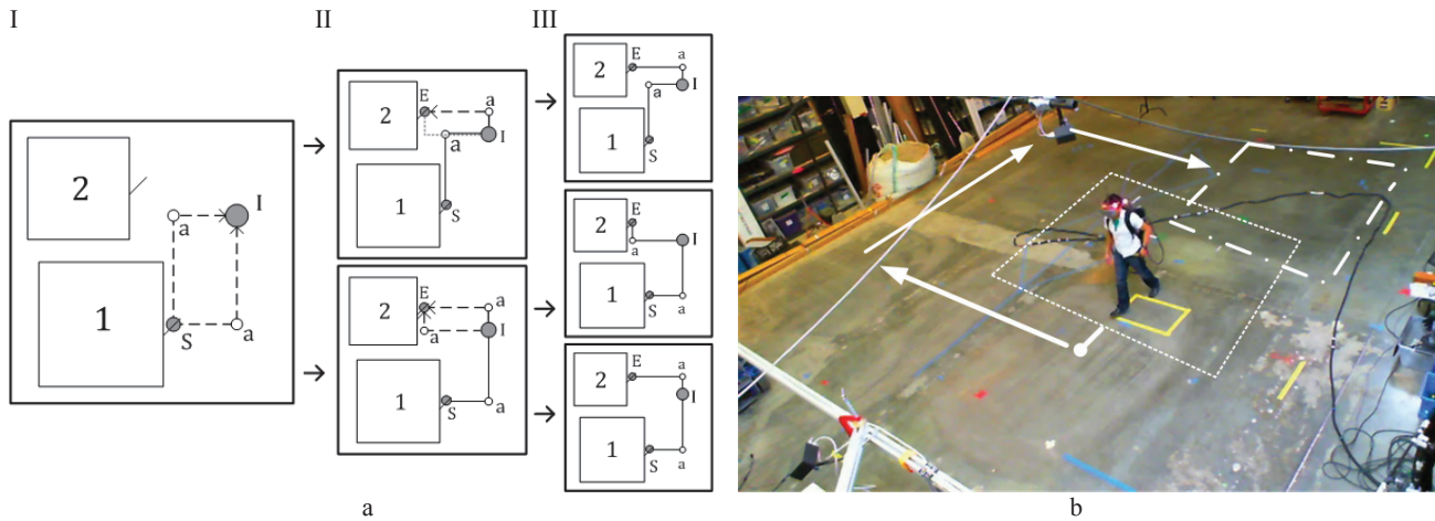
Figure 2: The path generation: (a) The algorithm has 3 main stages: I – random selection of the intermediate point I and additional points a, II – selection of the closest end-point E, III – random selection of the additional points between I and E. (b) An example of a simple path a user takes in our VE.
