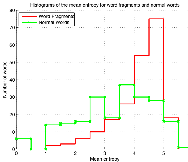
Fig. 1. Histograms of the mean entropy across the ASR output lattice of the word hypotheses during word fragments and normal words. 211 samples each of word fragments and normal words were taken from the San Diego corpus [3].
