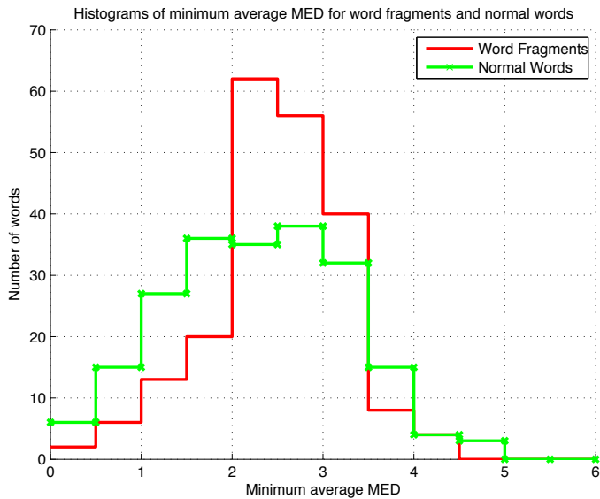
Fig. 3. Histograms of the minimum average MED across the ASR output lattice during word fragments and normal words. 211 samples each of word fragments and normal words were taken from the San Diego corpus [3].
