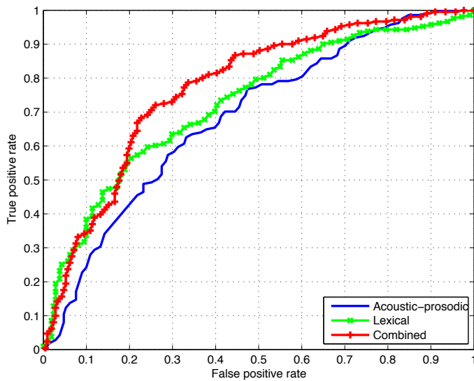
Fig. 4. ROC curves for classification experiments using acoustic-prosodic, lexical and combined feature sets (without dimensionality reduction). The areas under the curves are 0.686, 0.728 and 0.773 respectively.
