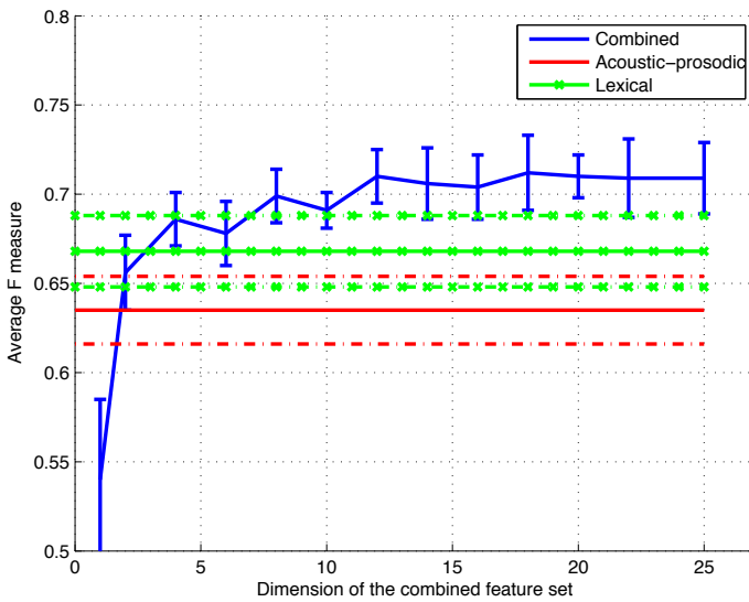
Fig. 5. Classification performance using a combined feature set of varying dimension. Also shown are the average F measures for the complete set of acoustic-prosodic and lexical features, with a \pm 1 standard deviation margin.
