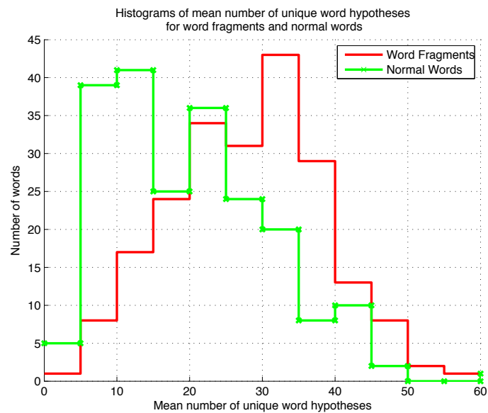
Fig. 2. Histograms of the mean number of unique word hypotheses across the ASR output lattice during word fragments and normal words. 211 samples each of word fragments and normal words were taken from the San Diego corpus [3].
