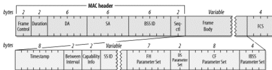
Figure 4-41. Probe Response frame
