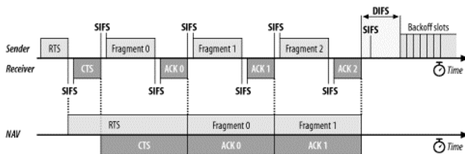
Figure 3-8. Fragmentation burst
