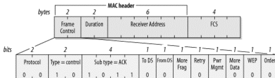
Figure 4-17. ACK frame
