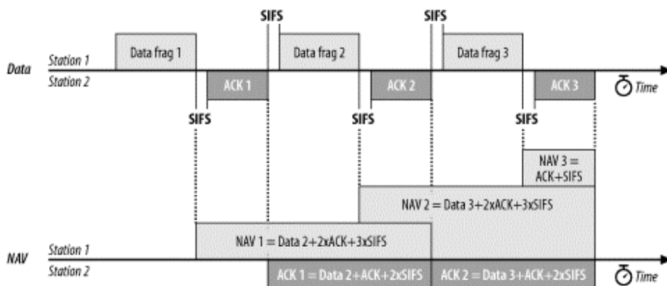
Figure 3-16. Fragmentation
