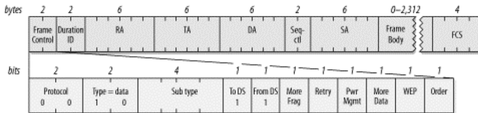
Figure 4-11. WDS frames
