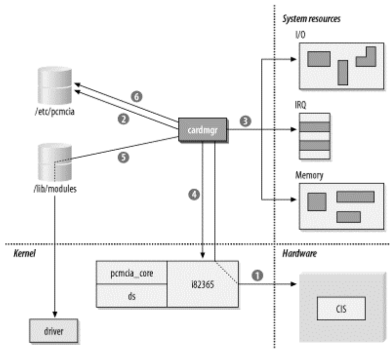
Figure 13-1. Linux PCMCIA configuration system
