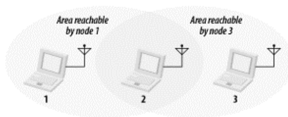
Figure 3-2. Nodes 1 and 3 are "hidden"
