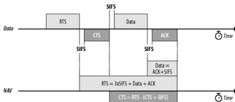
Figure 3-17. RTS/CTS lockout
