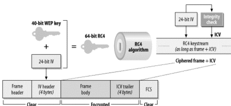
Figure 5-3. WEP operations
