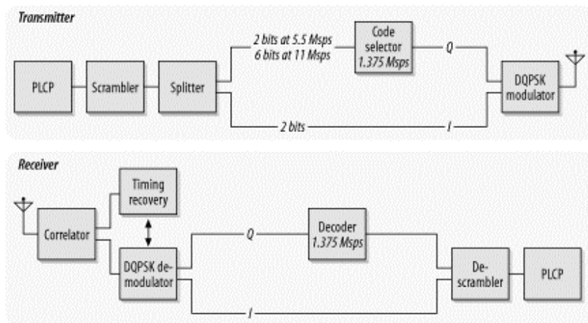
Figure 10-28. HR/DSSS transceiver
