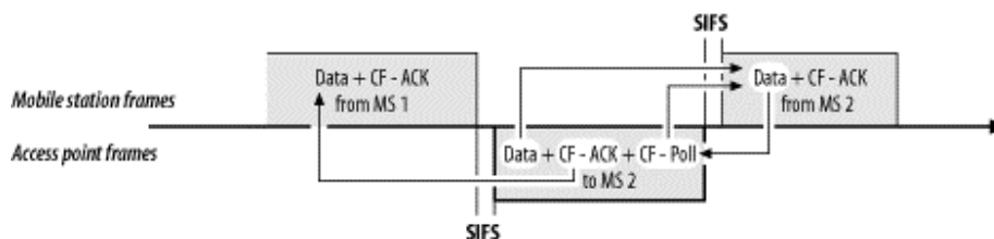
Figure 8-4. Usage of Data+CF-Ack+CF-Poll
