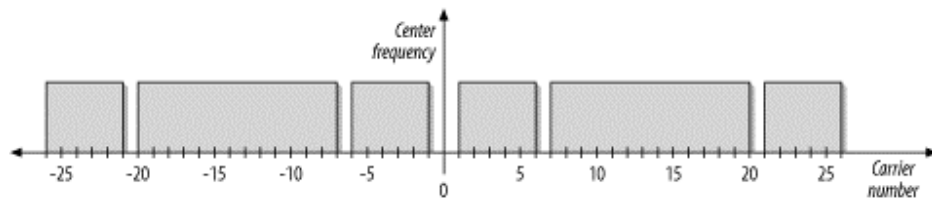
Figure 11-8. Structure of an OFDM channel
