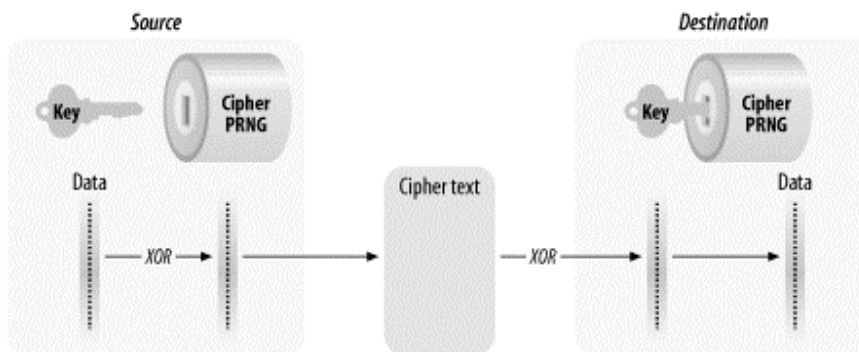
Figure 5-2. Keyed stream cipher operation
