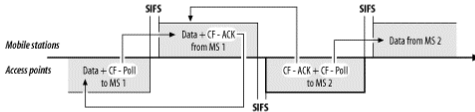
Figure 8-6. CF-Ack+CF-Poll usage
