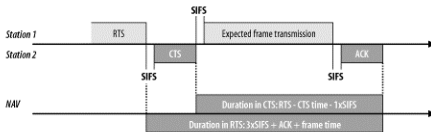
Figure 4-16. CTS duration
