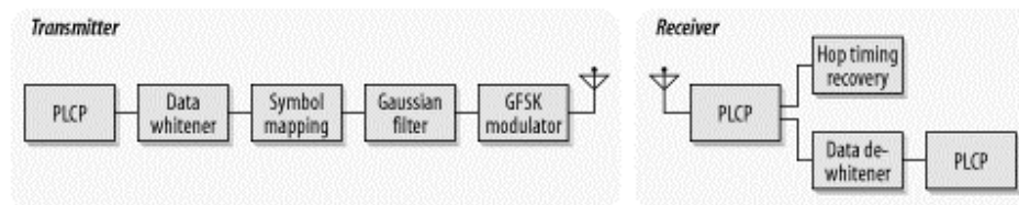
Figure 10-10. Frequency-hopping transceiver
