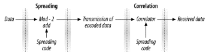
Figure 10-13. Chipping
