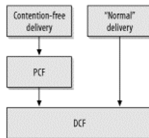
Figure 3-4. MAC coordination functions
