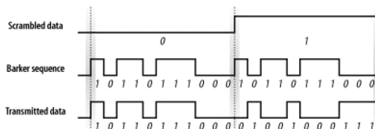
Figure 10-14. Encoding with the Barker word
