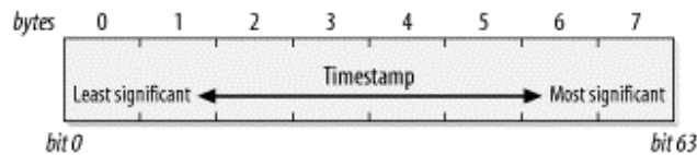
Figure 4-28. Timestamp field
