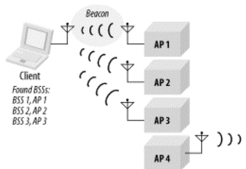
Figure 7-2. Passive scanning
