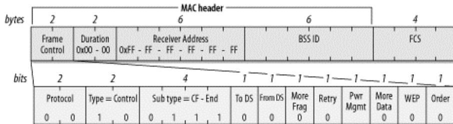
Figure 8-7. CF-End frame
