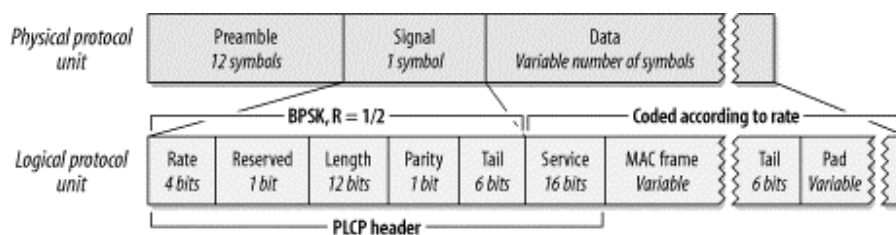
Figure 11-11. OFDM PLCP framing format
