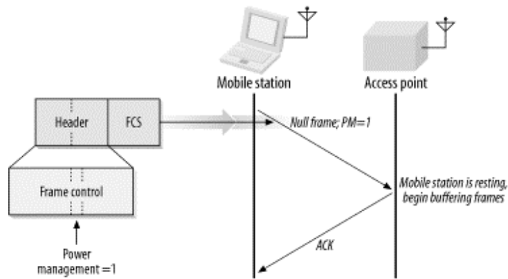
Figure 4-7. Data frame of subtype Null
