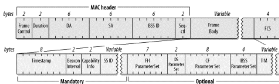
Figure 4-39. Beacon frame
