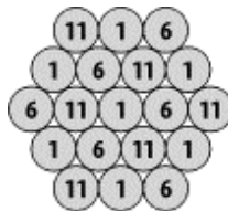
Figure 15-6. Frequency planning
