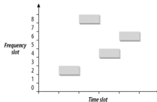
Figure 10-1. Frequency hopping
