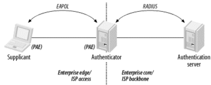
Figure 6-6. 802.1x architecture
