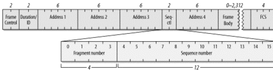
Figure 3-12. Sequence Control field
