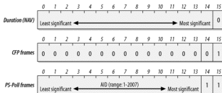
Figure 3-11. Duration/ID field
