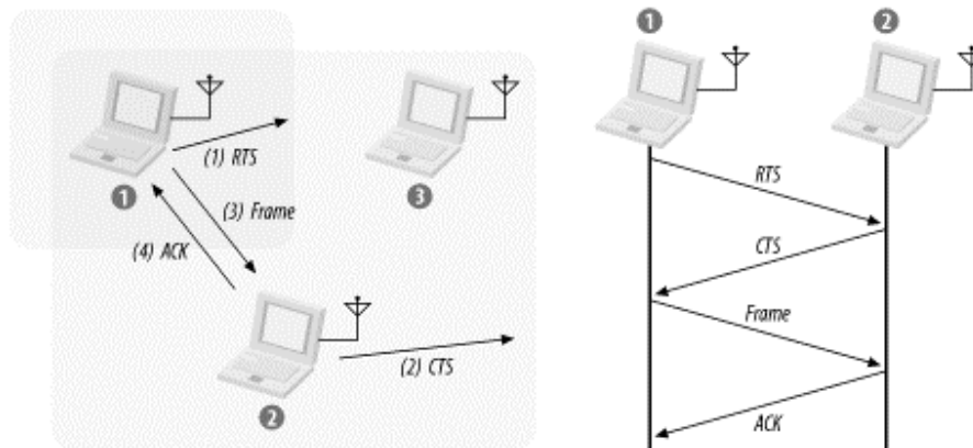
Figure 3-3. RTS/CTS clearing
