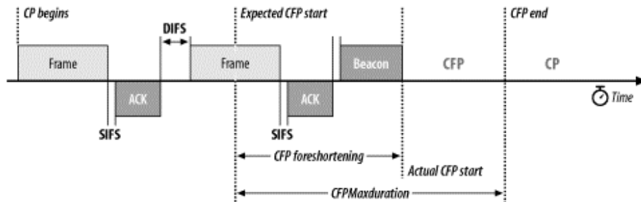
Figure 8-2. Data+CF-Ack and Data+CF-Poll usage
