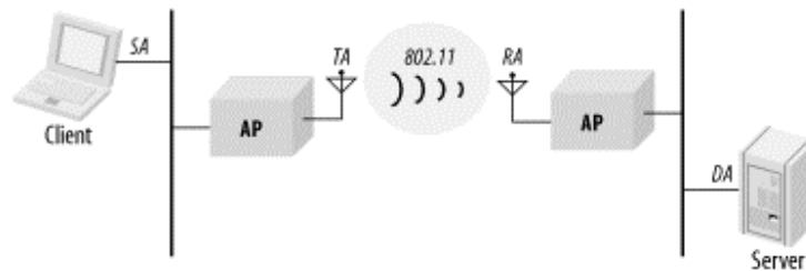
Figure 4-6. Wireless distribution system
