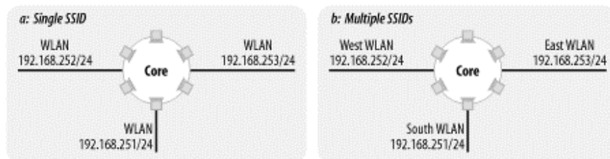
Figure 15-4. Noncontiguous deployments
