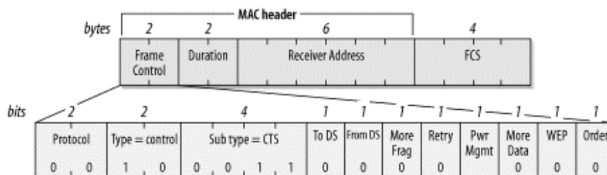
Figure 4-15. CTS frame
