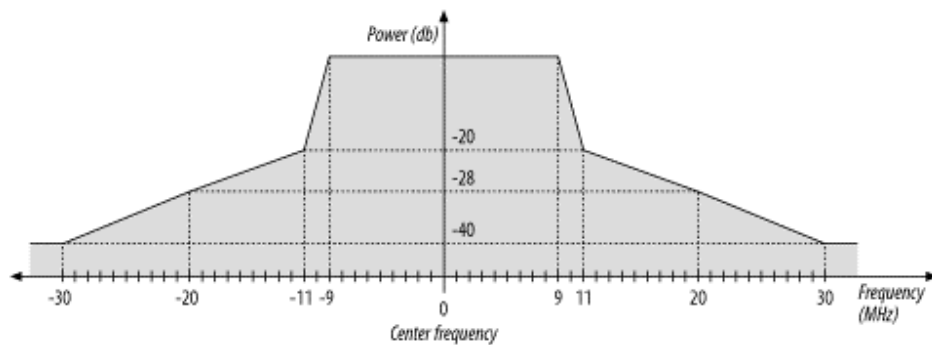
Figure 11-9. Transmit spectrum mask for 802.11a
