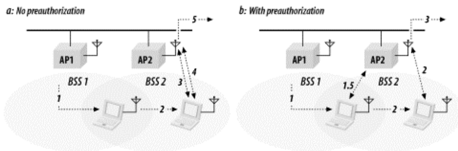
Figure 7-6. Time savings of preauthentication
