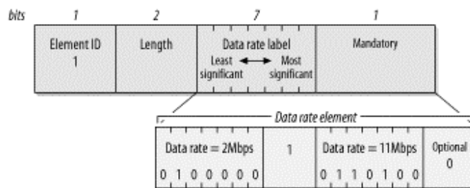
Figure 4-33. Supported Rates information element
