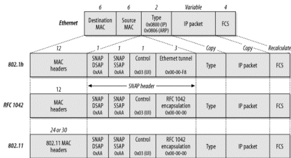
Figure 3-13. IP encapsulation in 802.11
