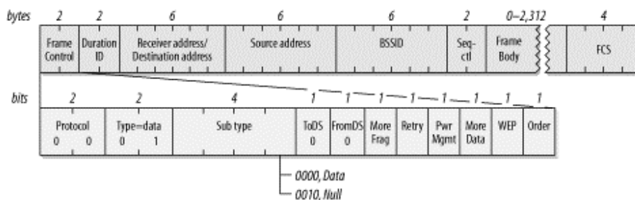
Figure 4-8. IBSS data frame
