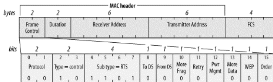
Figure 4-13. RTS frame
