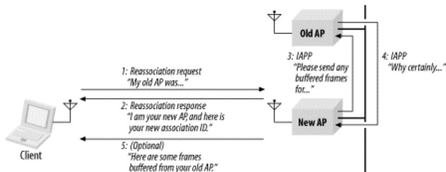
Figure 7-8. Reassociation procedure
