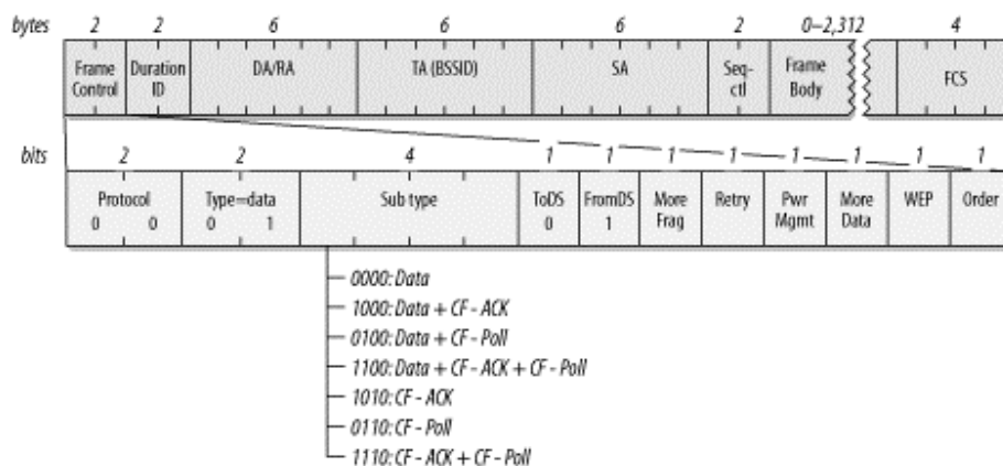
Figure 4-9. Data frames from the AP
