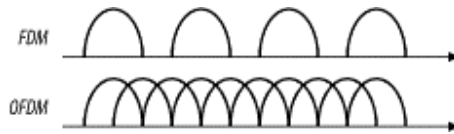
Figure 11-2. FDM versus OFDM
