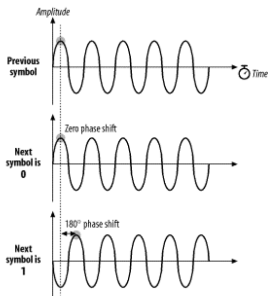
Figure 10-19. DBPSK encoding
