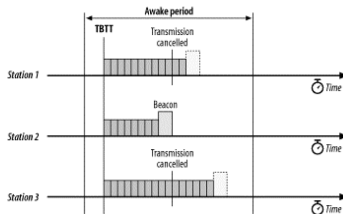
Figure 7-18. Distributed Beacon generation
