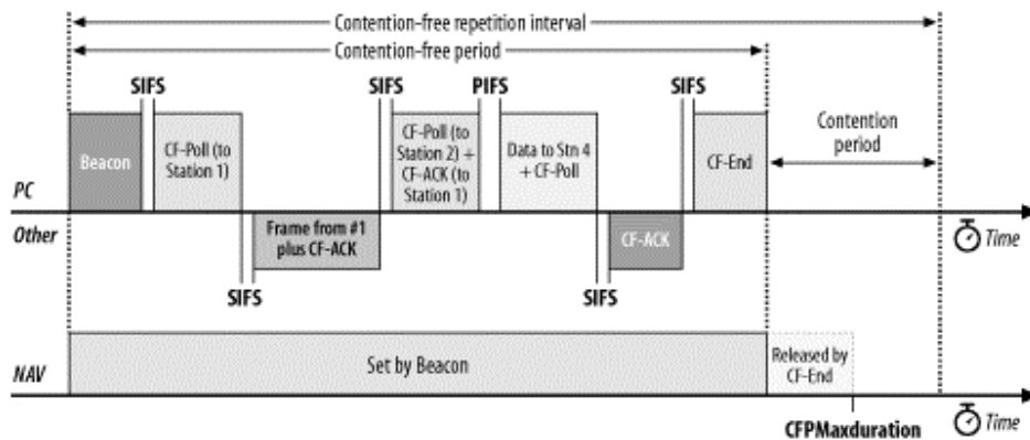
Figure 8-1. Using the PCF
