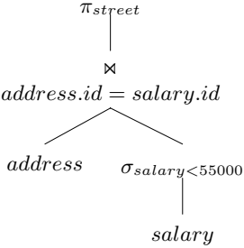
Fig. 13.2. Optimal query evaluation on unencrypted data
