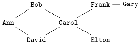
Fig. 4.7. An example of a privilege dependency graph
