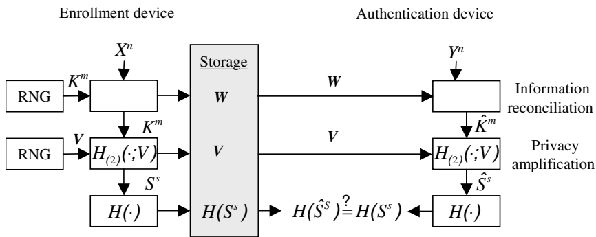
Fig. 27.4. The complete architecture based on information reconciliation and privacy amplification.
